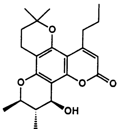
Dihydrocalanolide A
