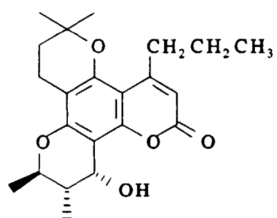
DIHYDROCALANOLIDE B
