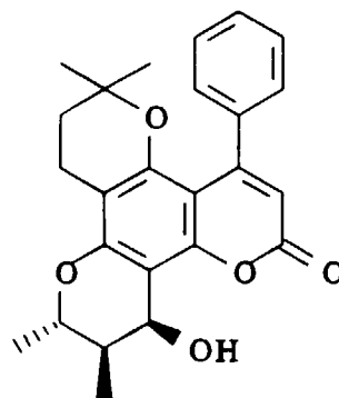
DIHYDROSOULATTROLIDE
