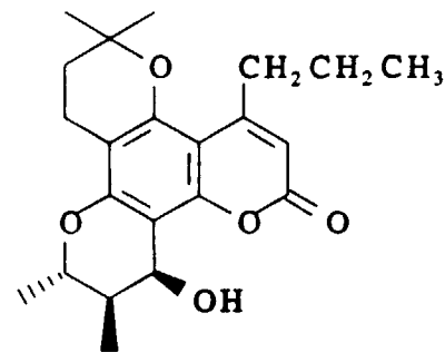
DIHYDROCOSTATOLIDE
