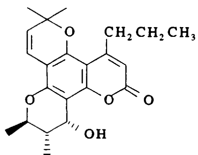
CALANOLIDE B
