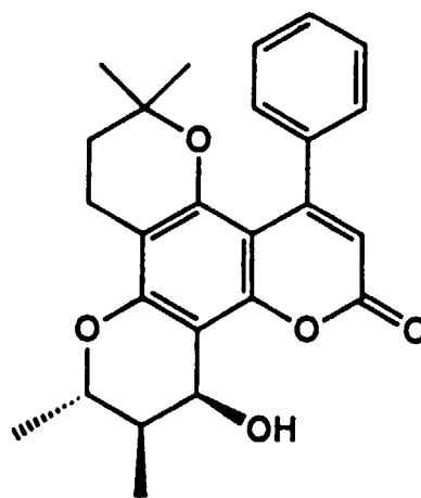
Dihydrosoulattrolide
