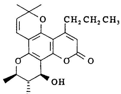
CALANOLIDE A
