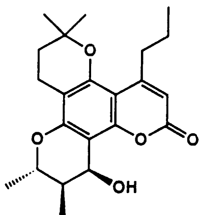
Dihydrocostatolide
