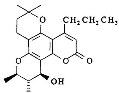
DIHYDROCALANOLIDE A
