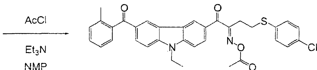
Compound 31
