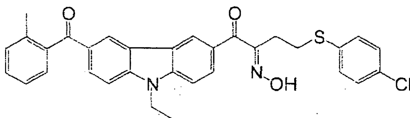
Compound B
