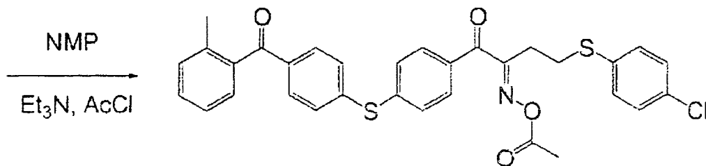
Compound 34
