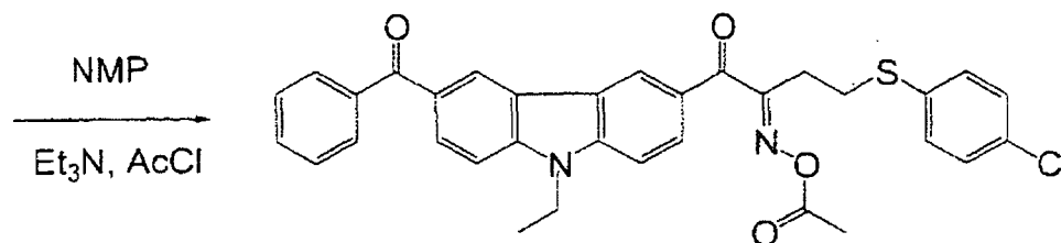
Compound 32
