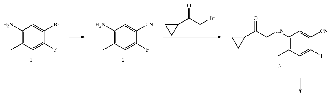
Scheme 2 Preparation of the Compound of formula (I) continued:
