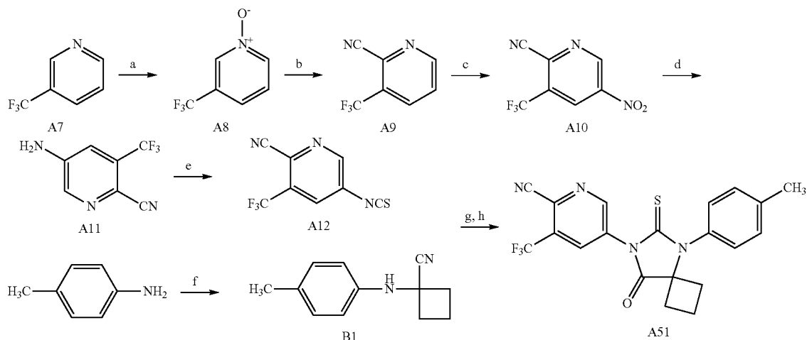
Scheme 2: Synthesis of A51
