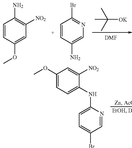
Scheme XII
