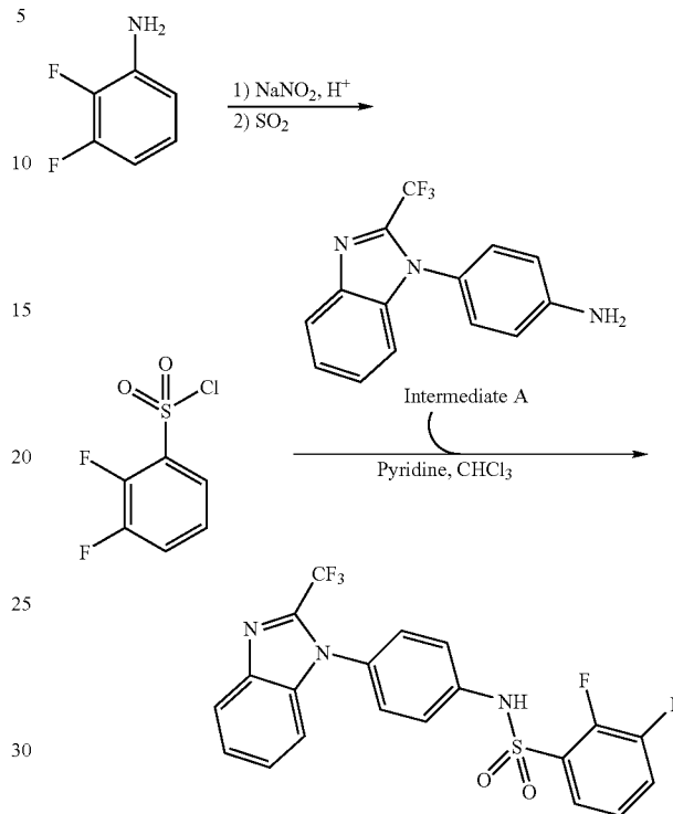
Compound 52
