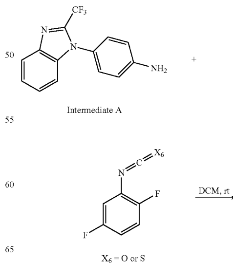
Scheme IV
