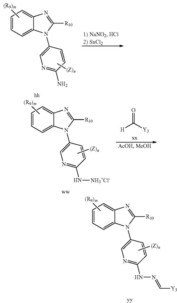
Scheme XVIII
