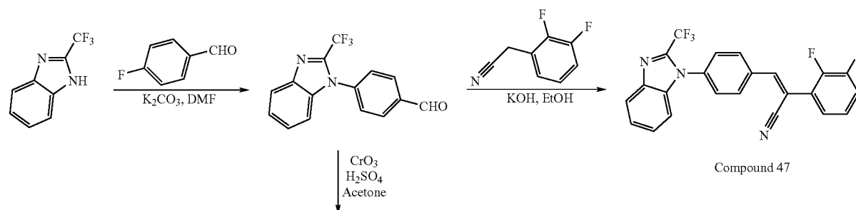
Scheme VII
