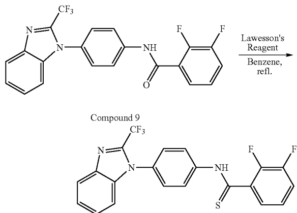
Compound 12
