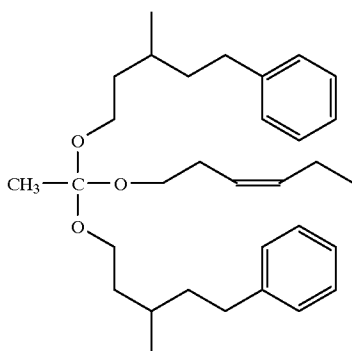
bis(5-phenyl-3-methylpentyl) cis-3-hexenyl orthoacetate
