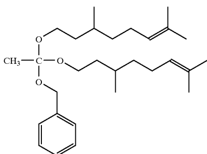
bis(citronellyl) benzyl orthoacetate
