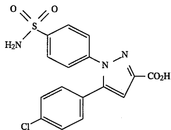
4-[4-(Aminosulfonyl)phenyl]-5-(4-chlorophenyl)-1H-pyrazole-3-carboxylate
