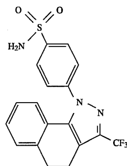
4,5-Dihydro-4-[3-trifluoromethyl]-1H-benz[g]indazol-1-yl]benzenesulfonamide
