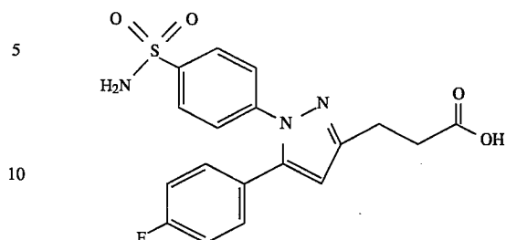
4-[4-(Aminosulfonyl)phenyl]-5-(4-fluorophenyl)-1H-pyrazole-3-propanoic acid
