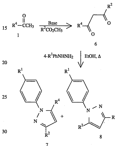
SCHEME II
