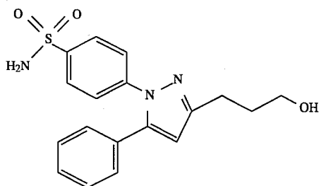
4-[5-Phenyl-3-(3-hydroxypropyl)-1H-pyrazol-1-yl]benzenesulfonamide
