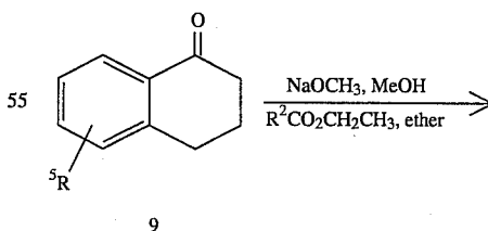
Scheme III
