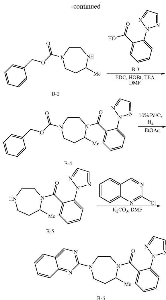
(R) or (S)-benzyl 5-methyl-1,4-diazepane-1-carboxylate (B-2)
