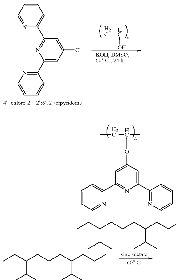
Scheme 1: Synthesis of metal induced supramolecular polymer gel
