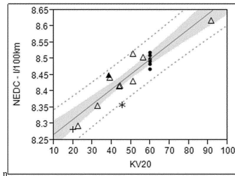
Figure 1. Bivariate Fit of NEDC Results
