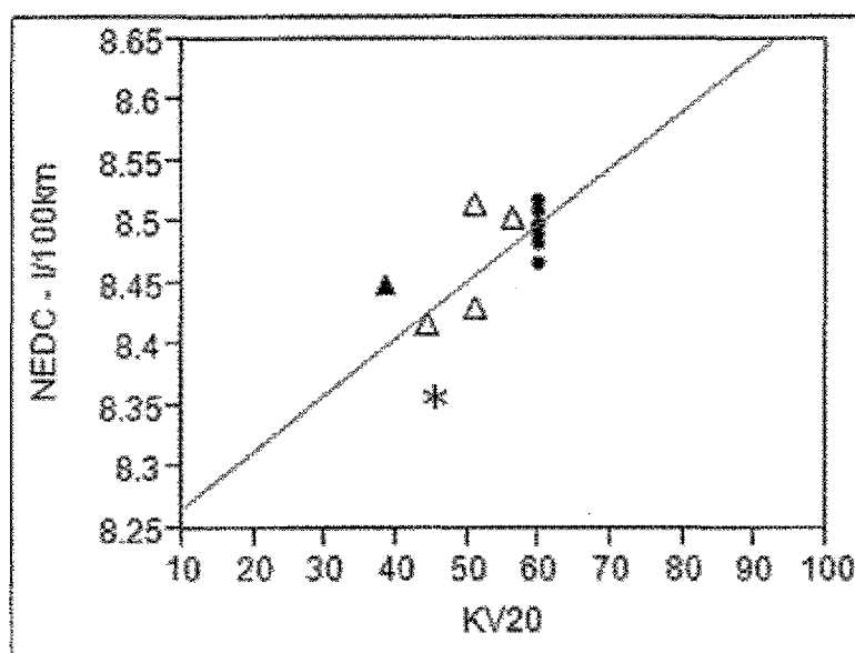
Figure 2. NEDC Fuel Consumption versus Kinematic Viscosity at 20°C
