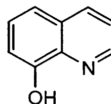
8-hydroxy-quinoline
