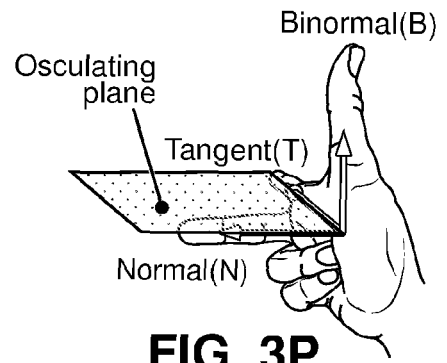
Right-hand rule
