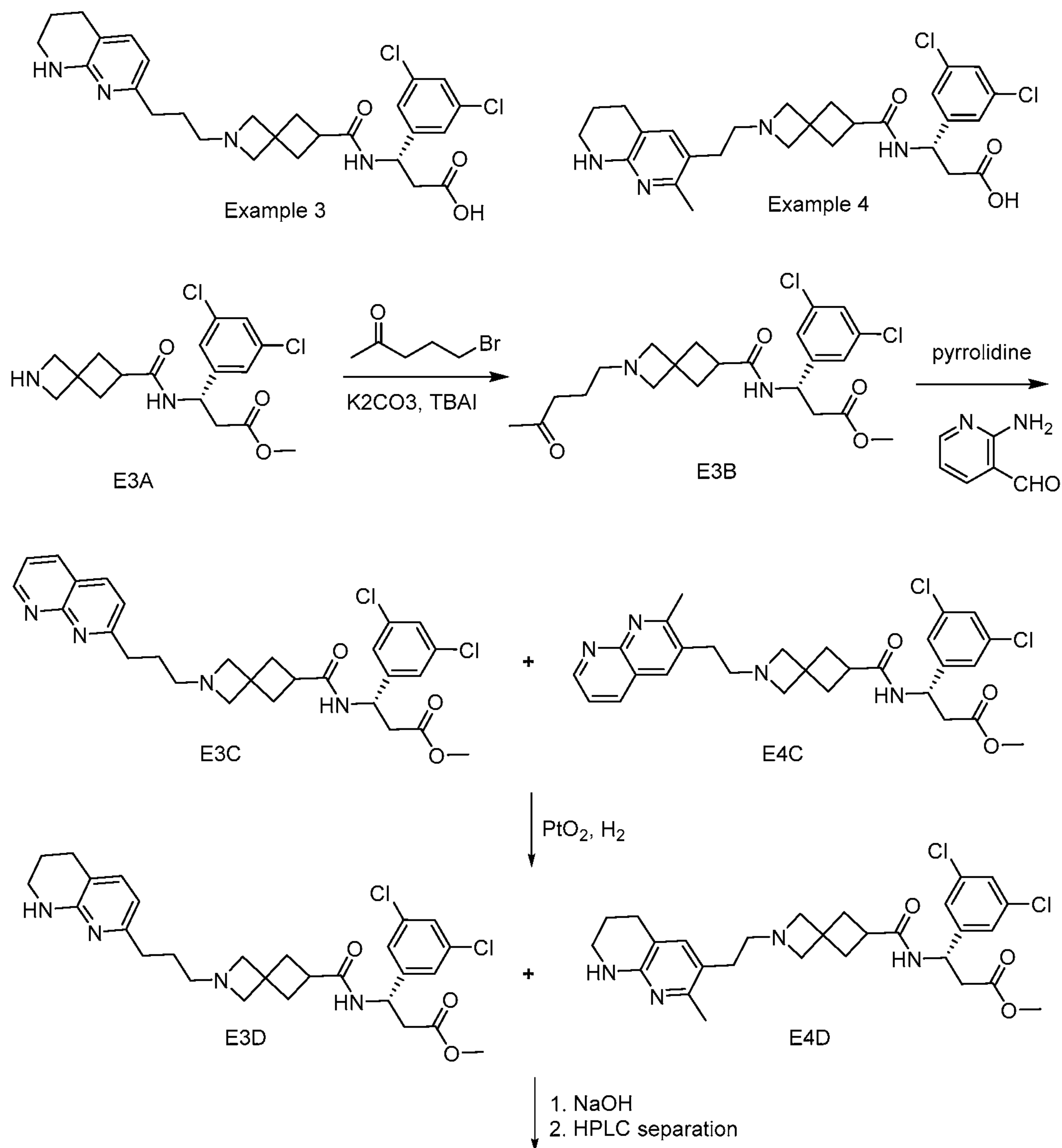
Example 3 and Example 4
