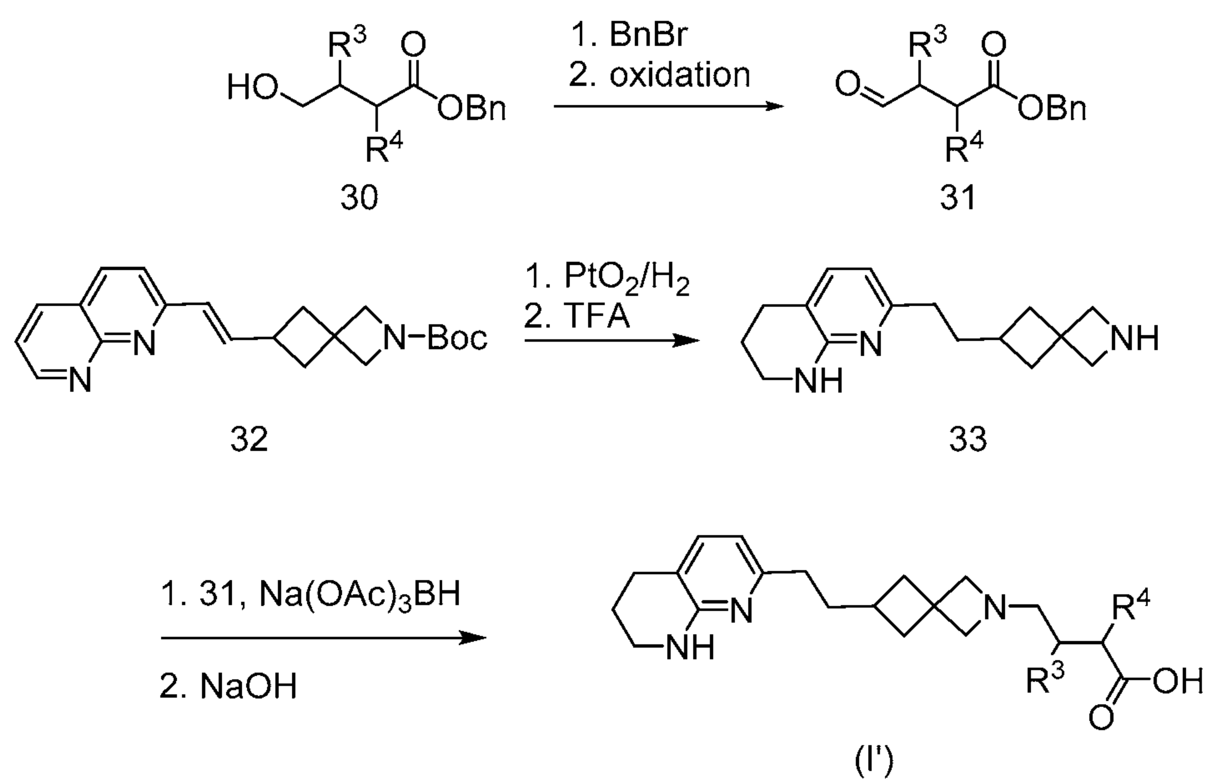
Scheme 8: General Scheme for preparation of Formula (I'), where X = (CH 2 ) 2 , Y = CH 2 , and A = bond
