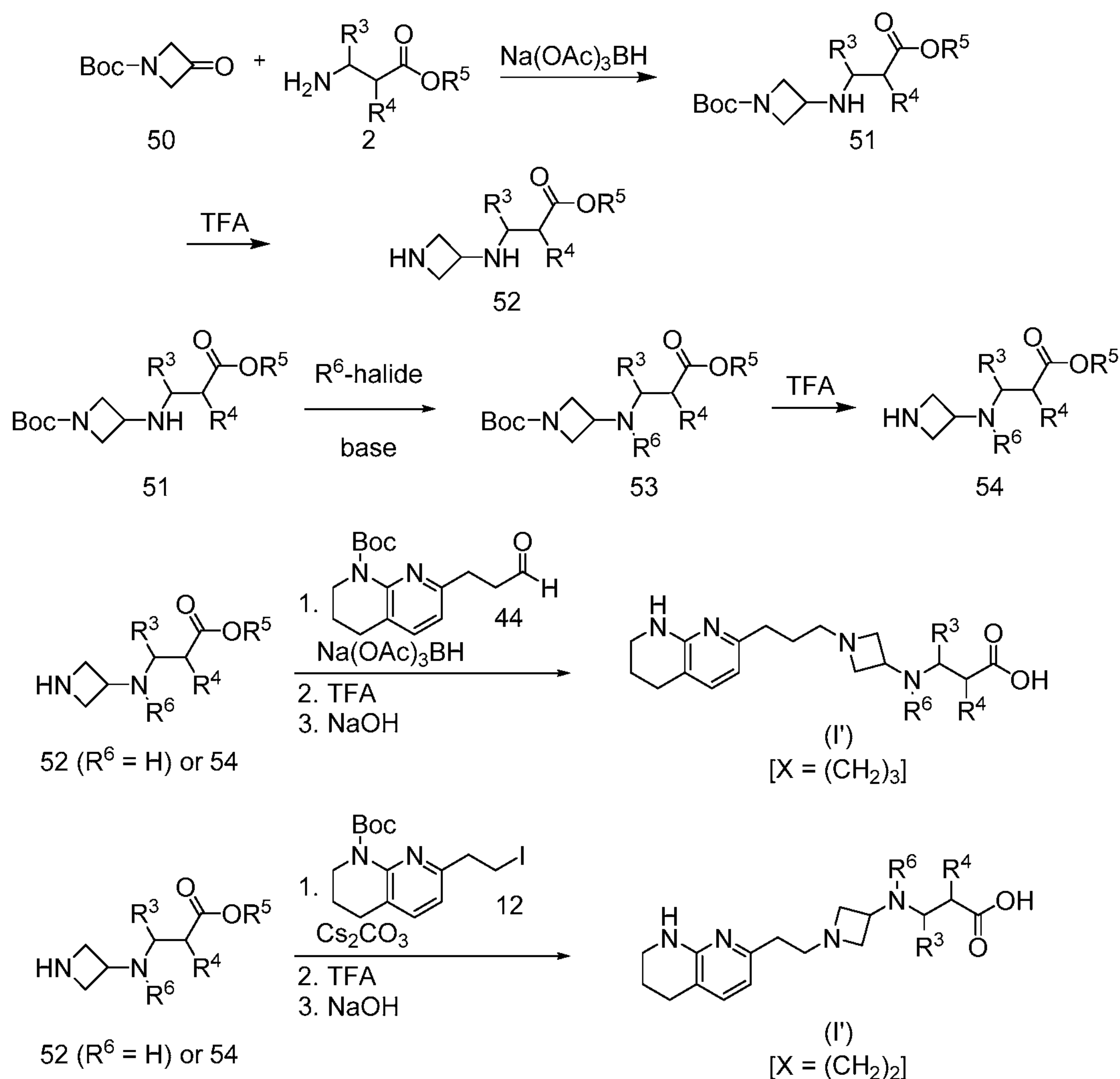
Scheme 11: General Scheme for preparation of Formula (I'), where X = (CH 2 ) 2-3 , Y = NR 6 , and A = bond
