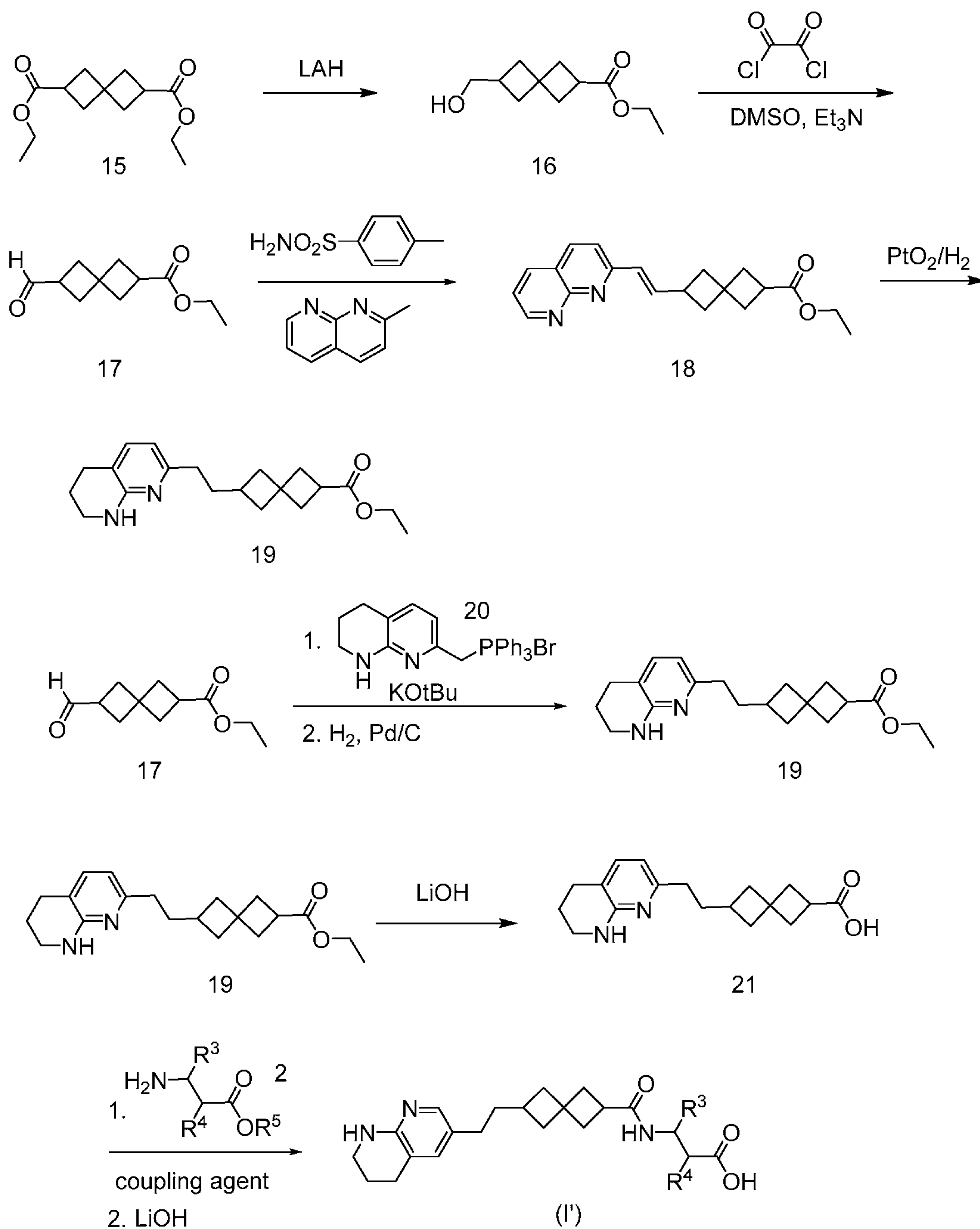
Scheme 5: General Scheme for preparation of Formula (I'), where X = (CH 2 ) 2 , R 1 = tetrahydronaphthyridine, and A = bond
