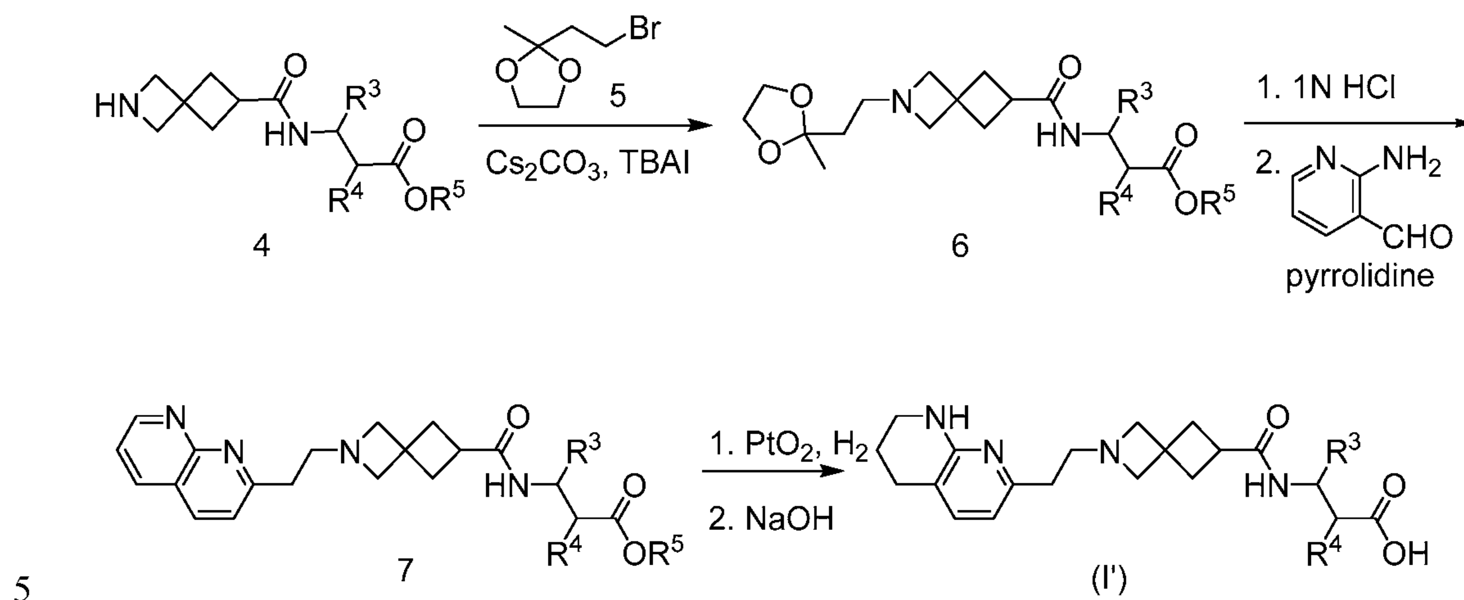
Scheme 2: General Scheme for preparation of Formula (I'), where R^1 = tetrahydronaphthyridine and X = CH_2CH_2 , Y = CONH, and A = bond
