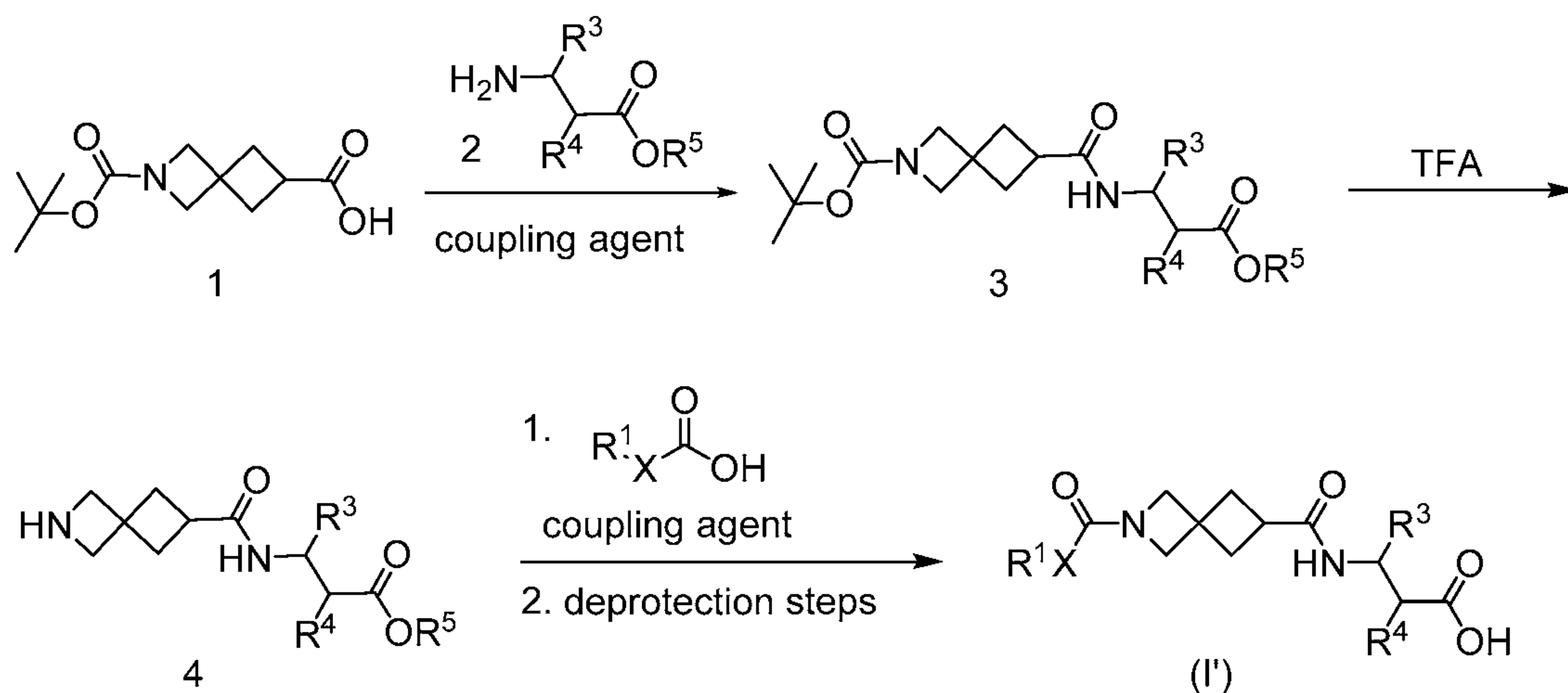
Scheme 1: General Scheme for preparation of Formula (I') where A = CO and Y = CONH
