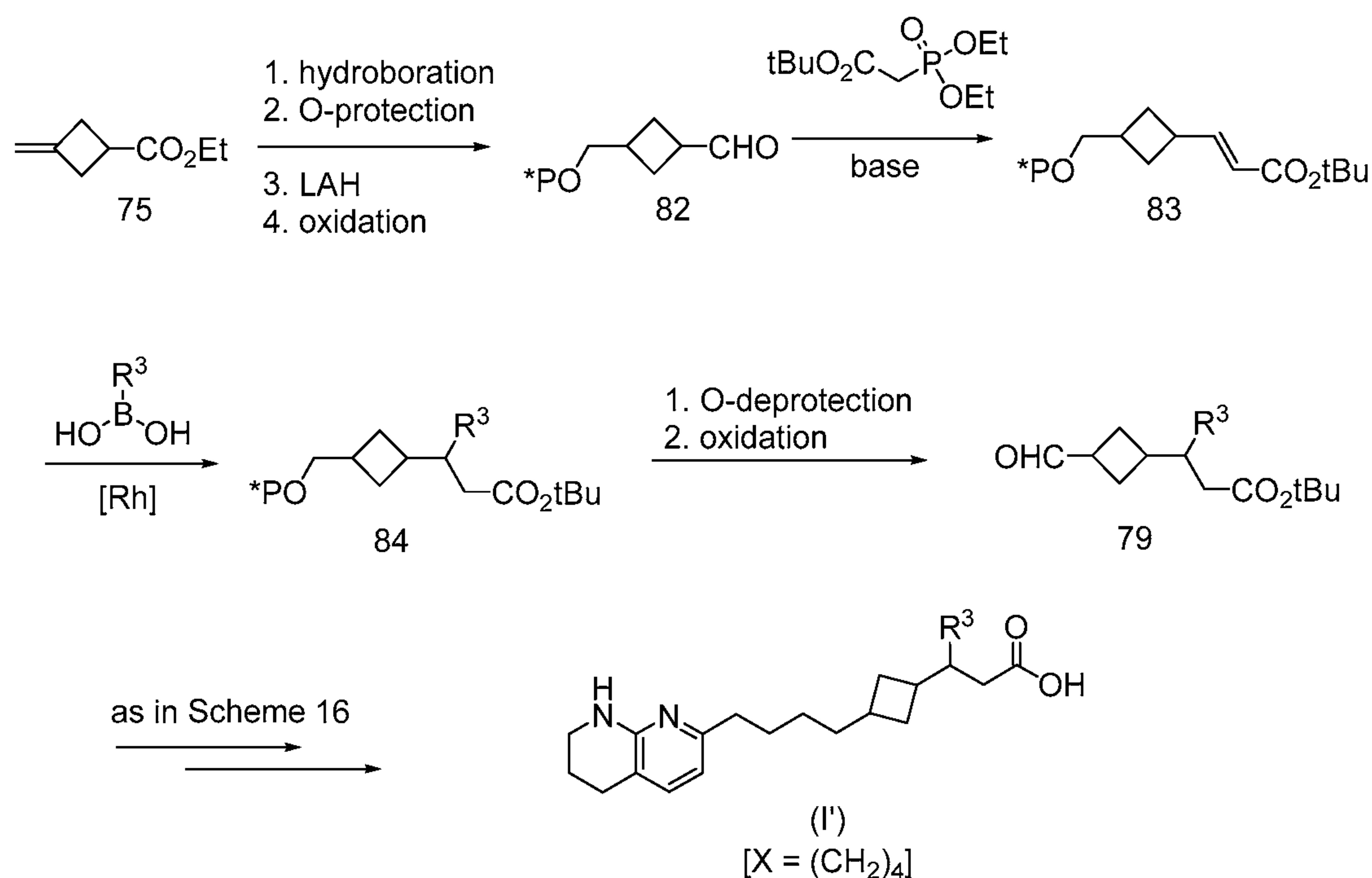
Scheme 17: General Scheme for preparation of Formula (I'), where X = (CH 2 ) 3-4 , Y = bond, and A = bond
