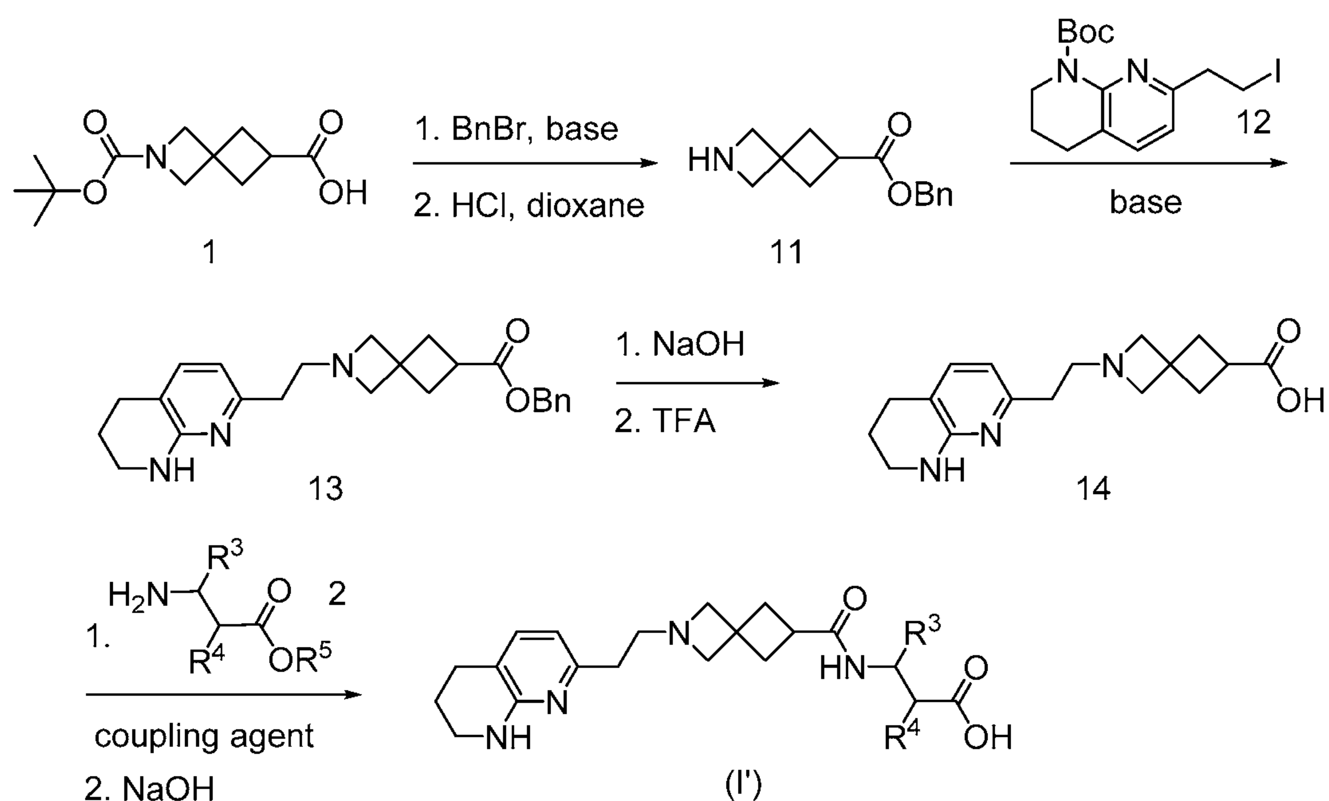
Scheme 4: General Scheme for preparation of Formula (I'), where X = (CH 2 ) 2 , Y = CONH, and A = bond
