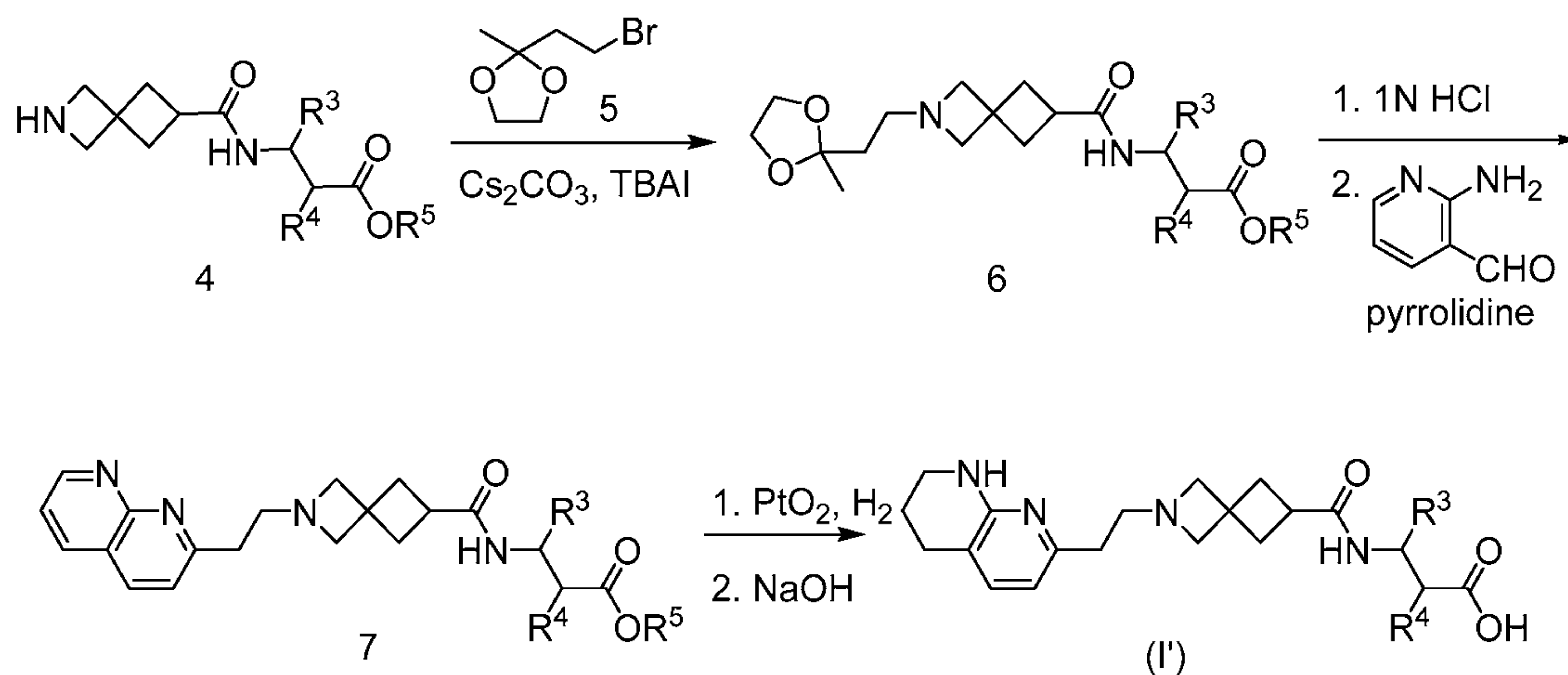
Scheme 2: General Scheme for preparation of Formula (I'), where \text{R}^1 = tetrahydronaphthylidene and X = \text{CH}_2\text{CH}_2 , Y = CONH, and A = bond
