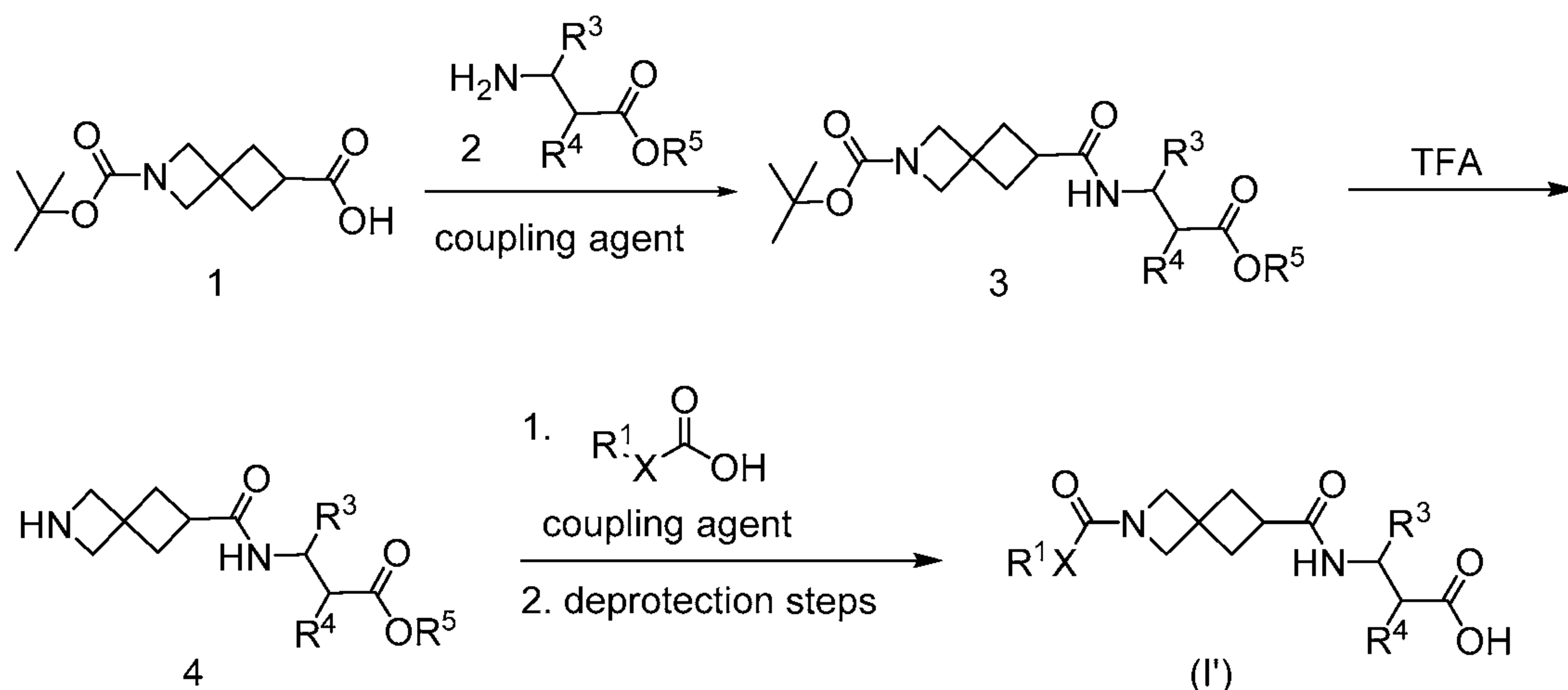
Scheme 2: General Scheme for preparation of Formula (I'), where R^1 = tetrahydronaphthyridine and X = CH_2CH_2 , Y = CONH, and A = bond
