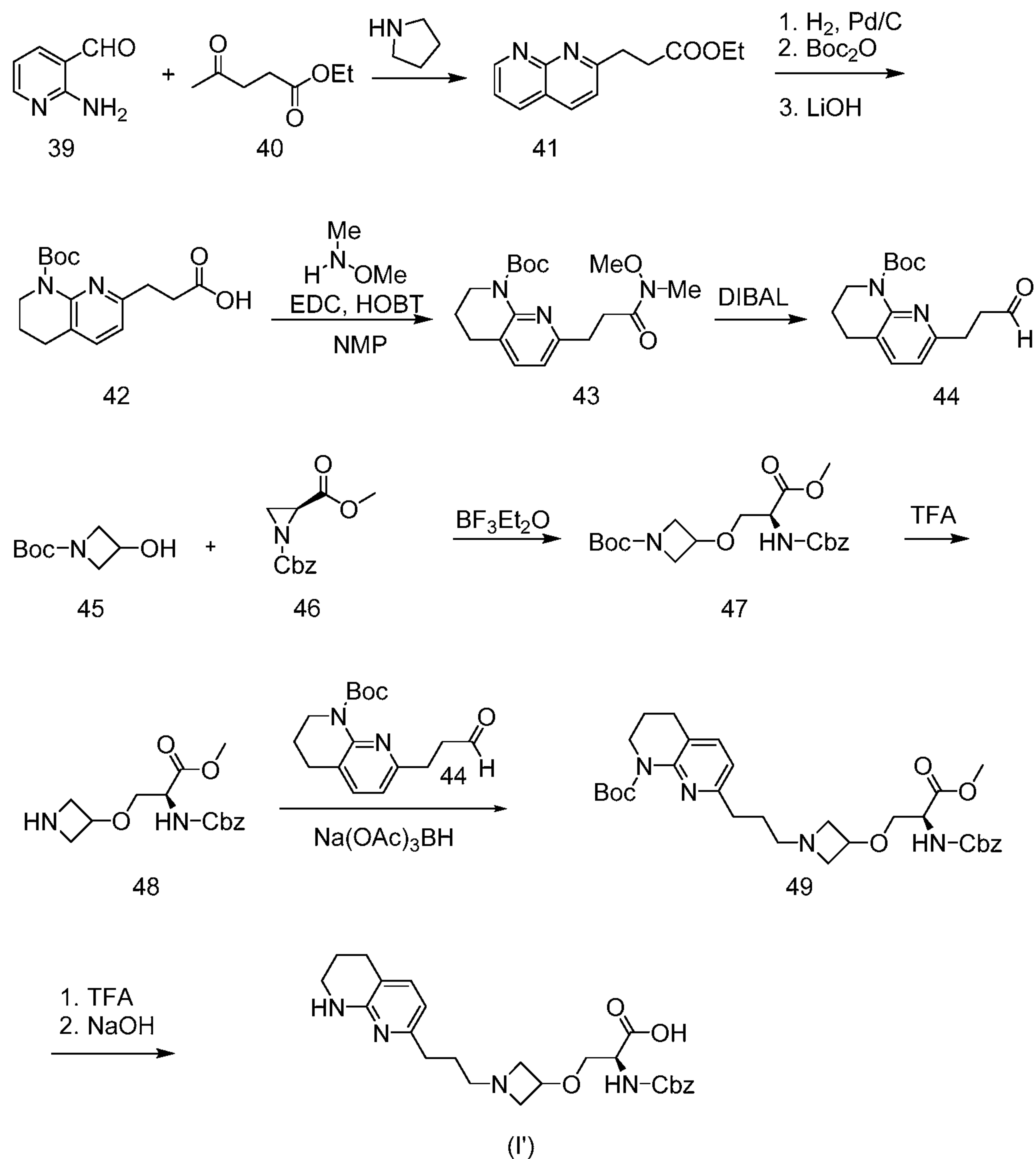
Scheme 10: General Scheme for preparation of Formula (I'), where X = (CH 2 ) 3 , Y = O, R 3 = H, and A = bond
