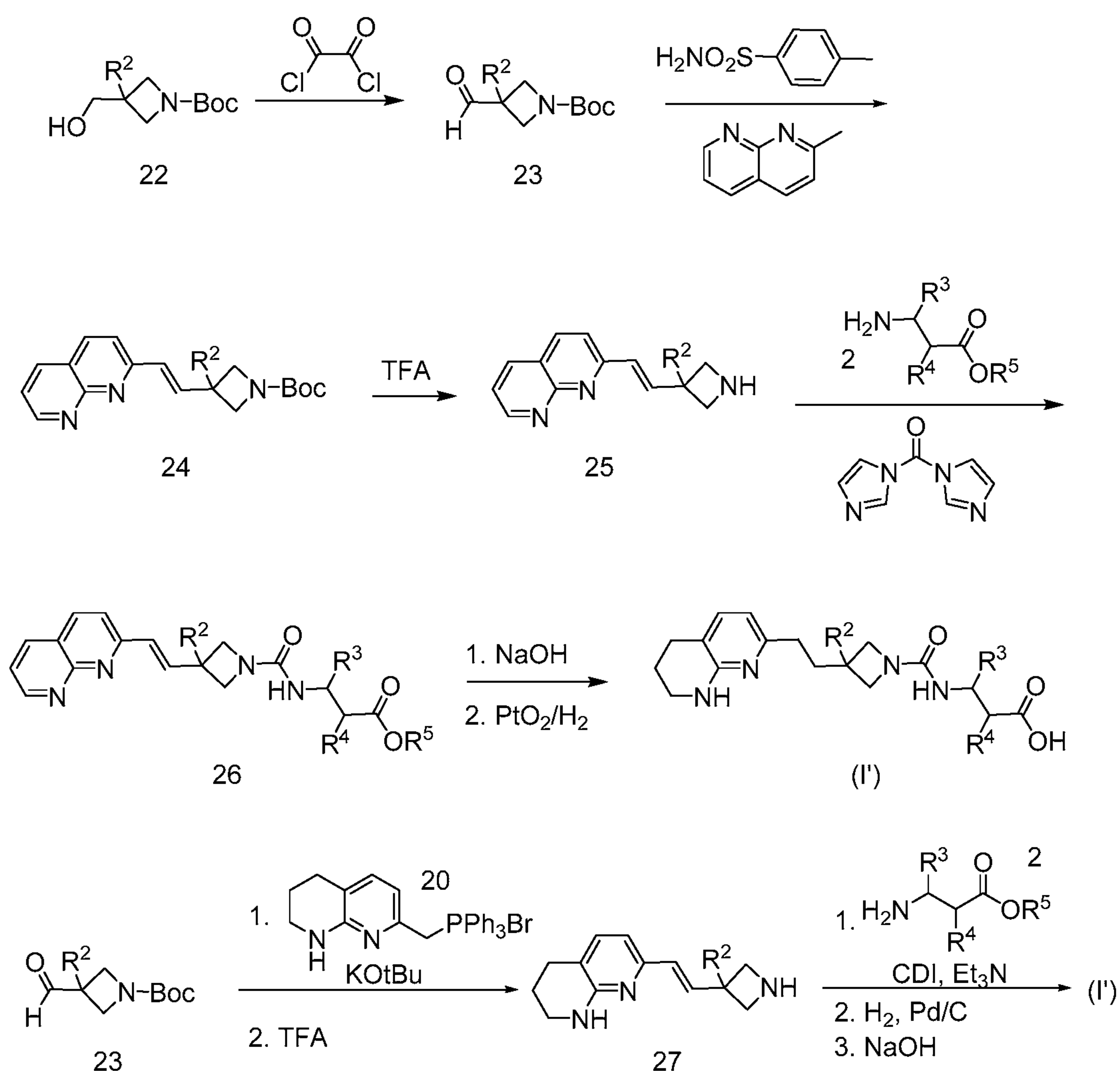
Scheme 6: General Scheme for preparation of Formula (I'), where X = (CH 2 ) 2 , Y = CONH, and A = bond
