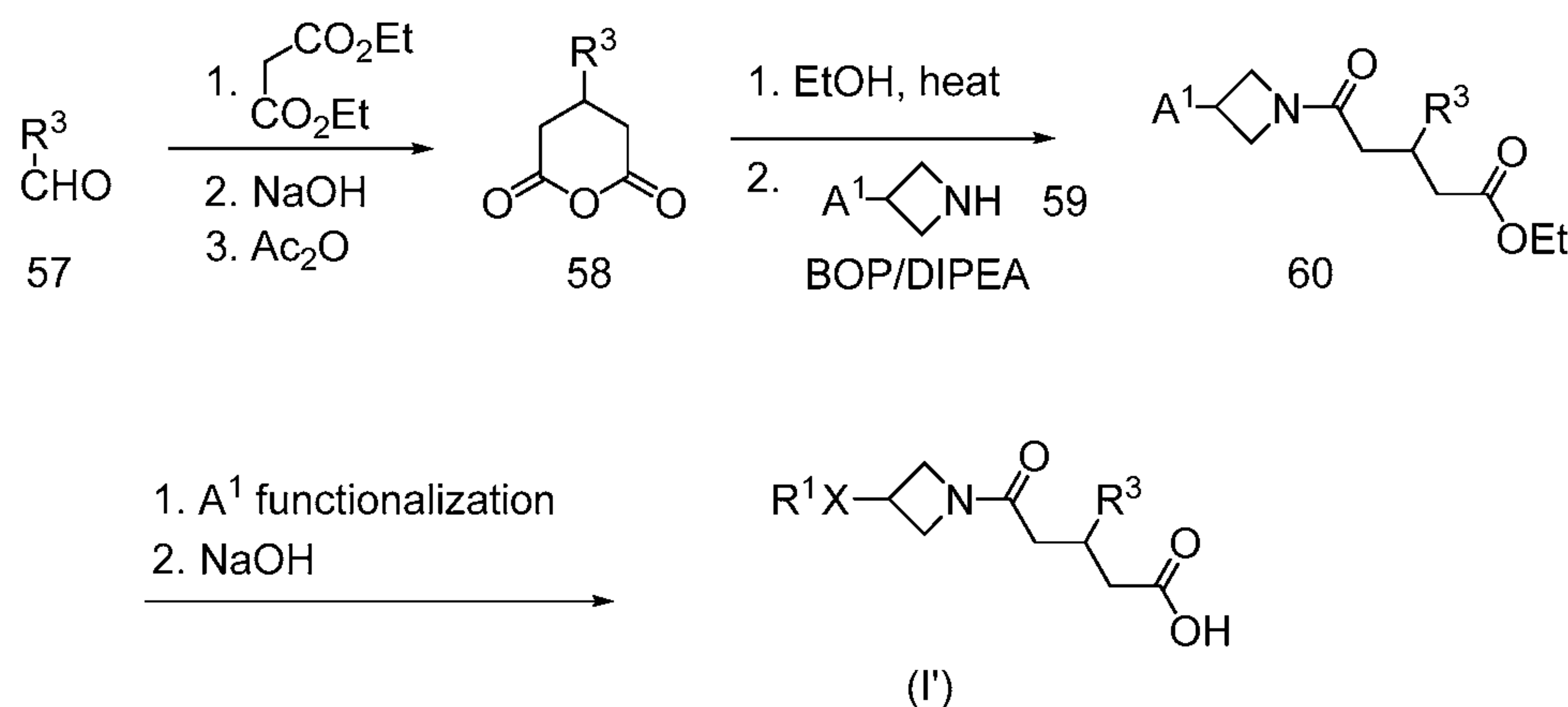
Scheme 13: General Scheme for preparation of Formula (I'), where X = (CH 2 ) 2-3 , Y = COCH 2 , R 4 = H, and A = bond
