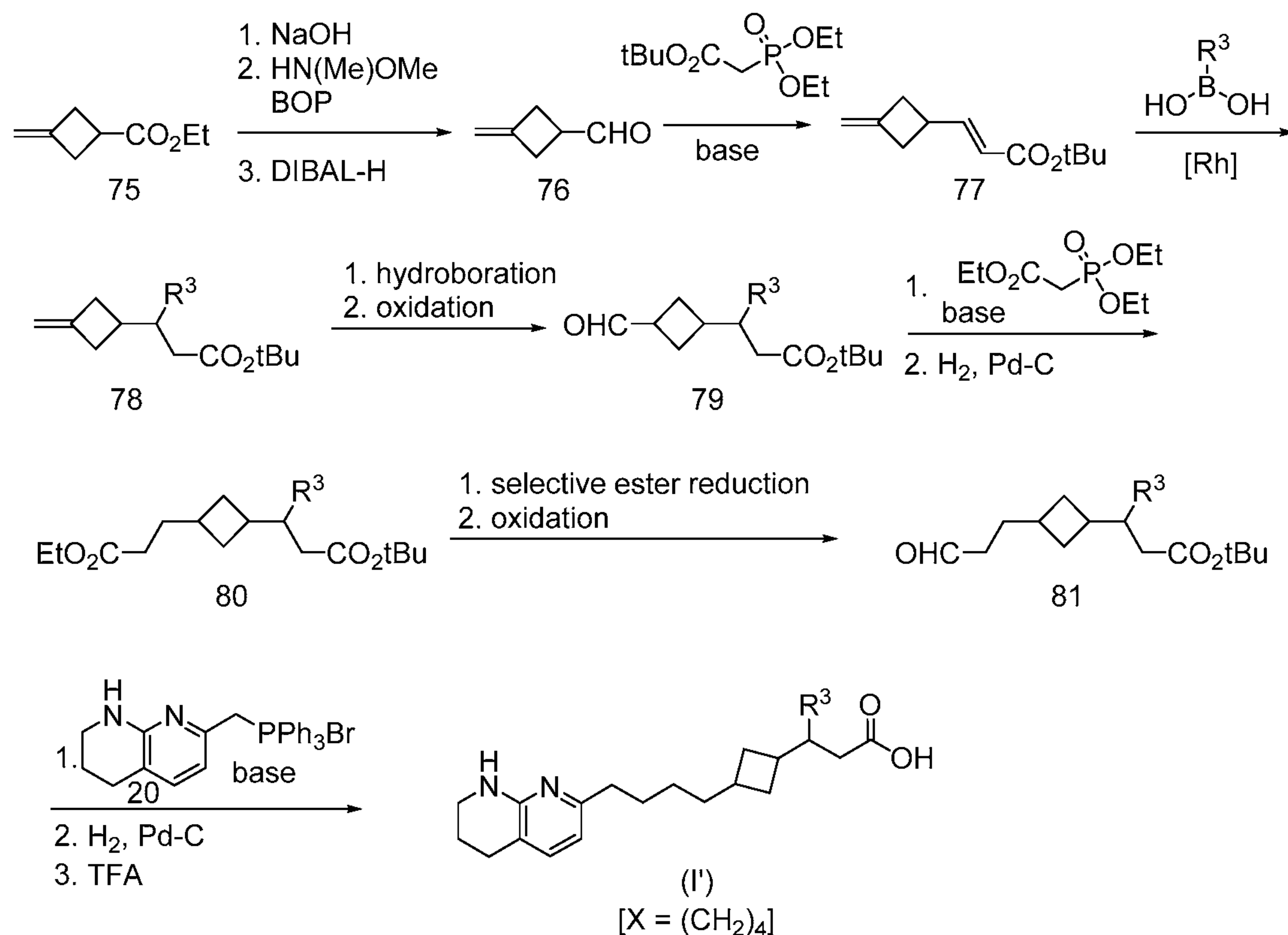
Scheme 17: General Scheme for preparation of Formula (I'), where X = (CH 2 ) 3-4 , Y = bond, and A = bond
