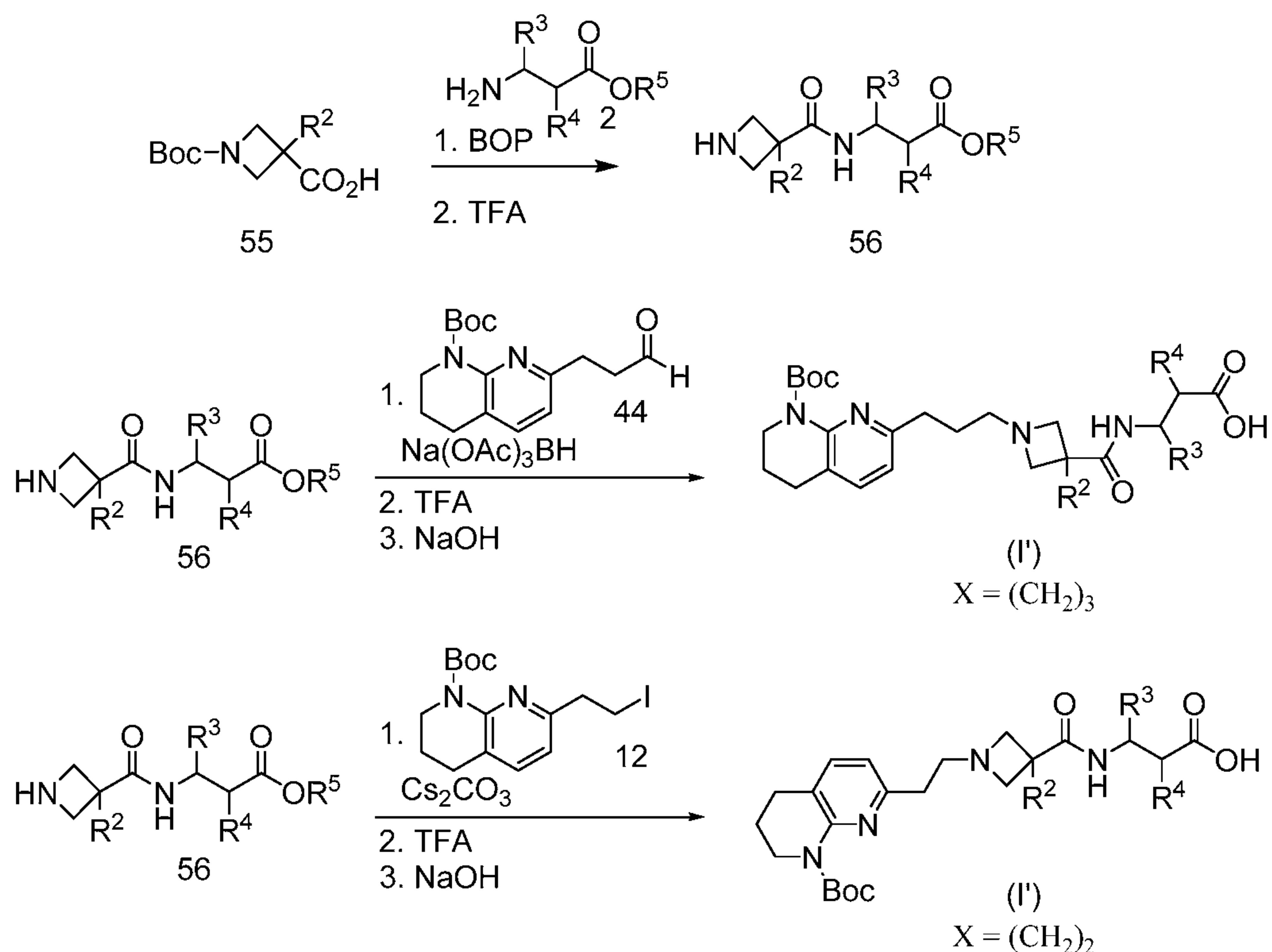
Scheme 12: General Scheme for preparation of Formula (I'), where X = (CH 2 ) 2-3 , Y = CONH, and A = bond
