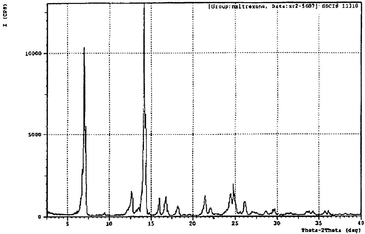
Figure 3. XRPD pattern of naltrexone lot 00-119-095 C (SSCI number 11310).
