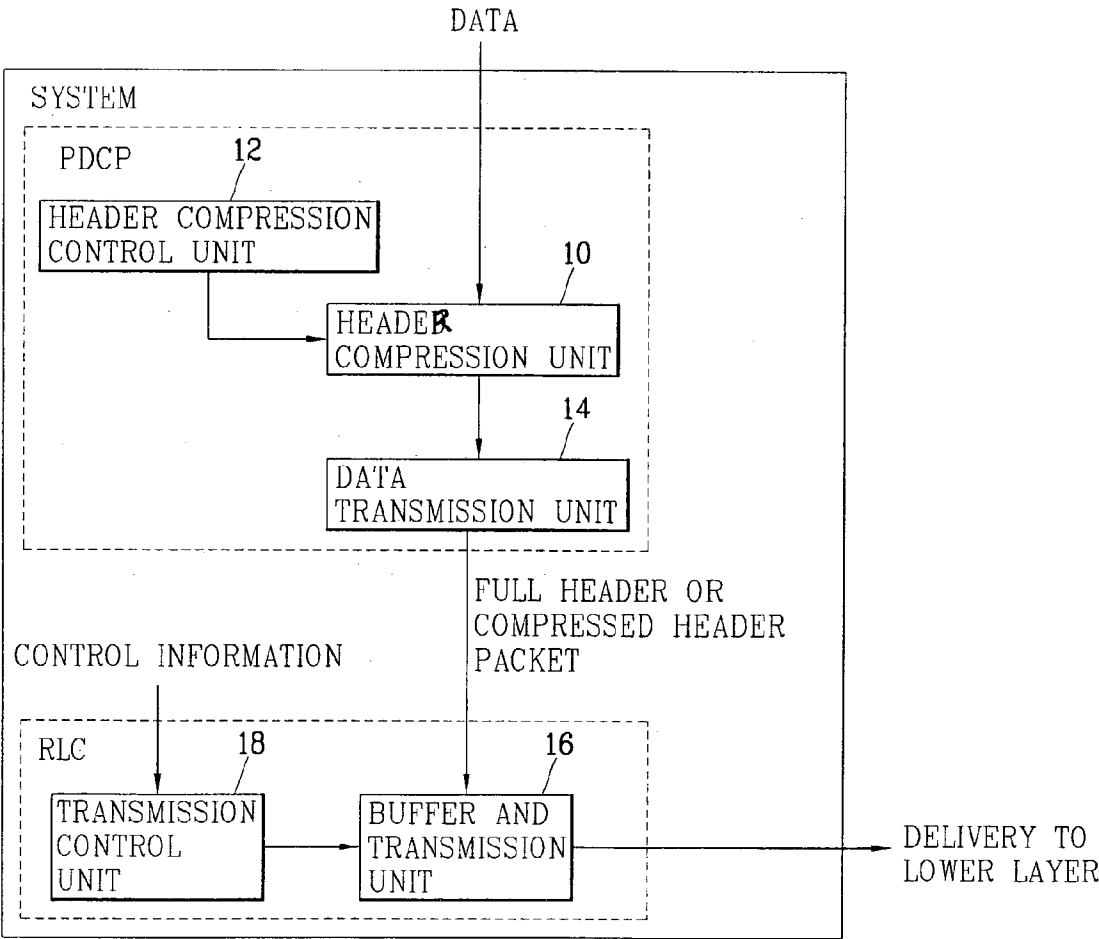
FIG. 2 RELATED ART
