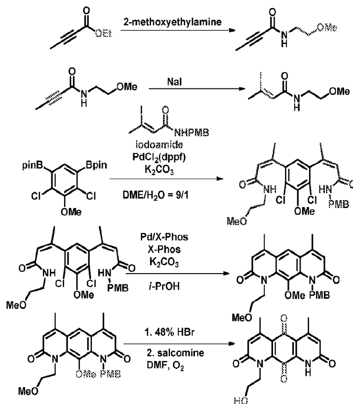
Scheme 7.4. Preparation of DNQ-P4.
