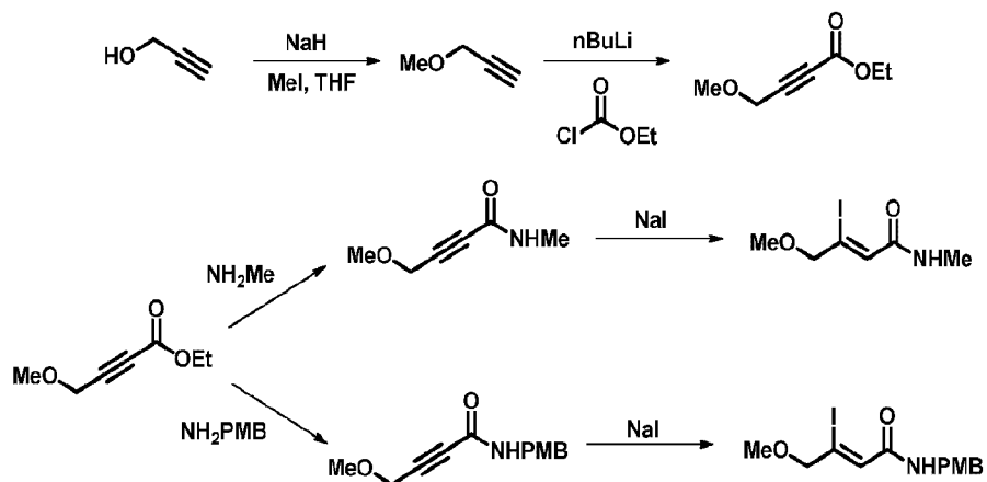
Scheme 7.2. Preparation of DNQ-P2 and DNQ-P3 Intermediates.
