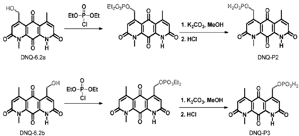
Scheme 7.3. Preparation of DNQ-P2 and DNQ-P3.
