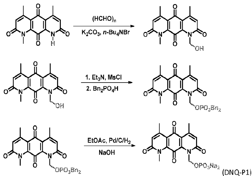
Scheme 7.1. Preparation of DNQ-P1.
