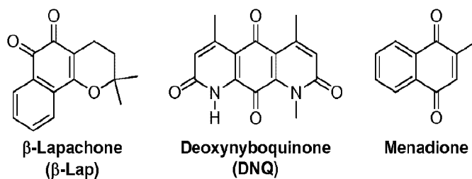
Scheme 1. Examples of Quinone Compounds.
