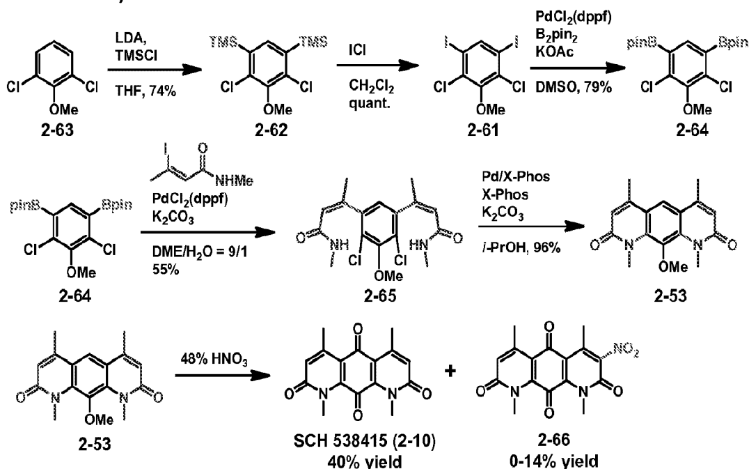
Scheme 1.12. Synthesis of SCH 538415.
