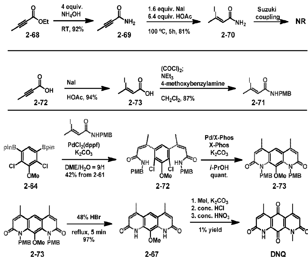
Scheme 1.13. Synthesis of DNQ by methylation of 2-67 .
