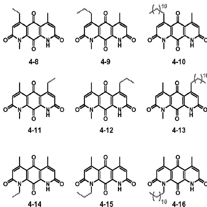
Scheme 4.1. Nine DNQ derivatives.
