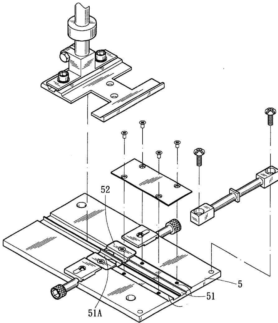
Fig. 5 (prior art)
