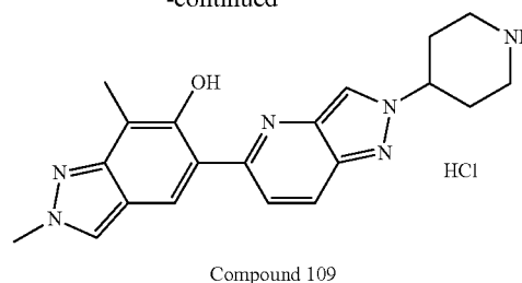
Compound 109
