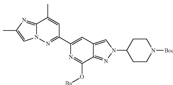
C140
