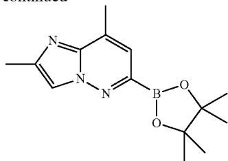
C139
