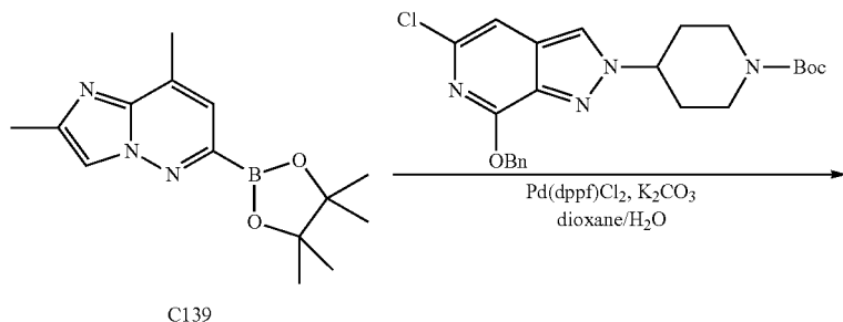
C139
