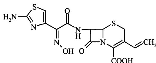
Form D
