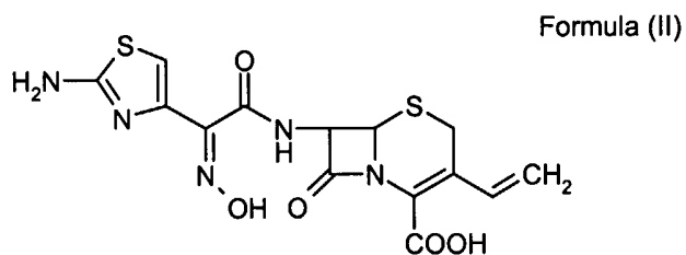
Cefdinir
