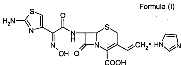
Cefdinir-Imidazole salt
