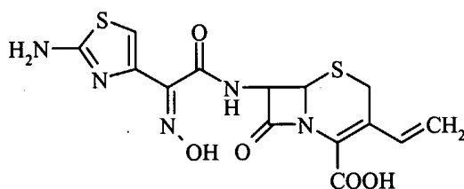
Form D
