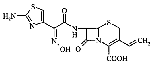
Form C
