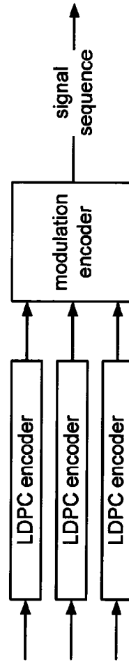
multilevel coded modulation Fig. 17C
