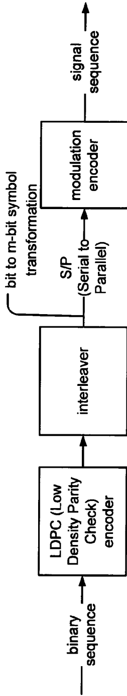
BICM (Bit Interleaved Coded Modulation) Fig. 17B
