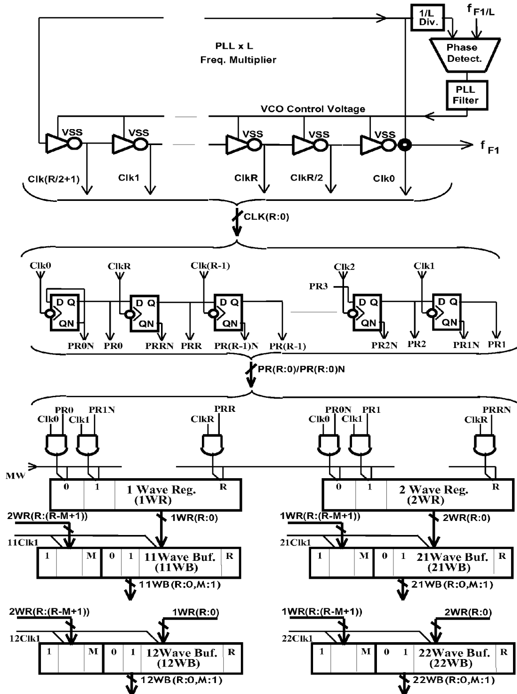
FIG.8 Wave Capturing including Edge Regions (WCER)
