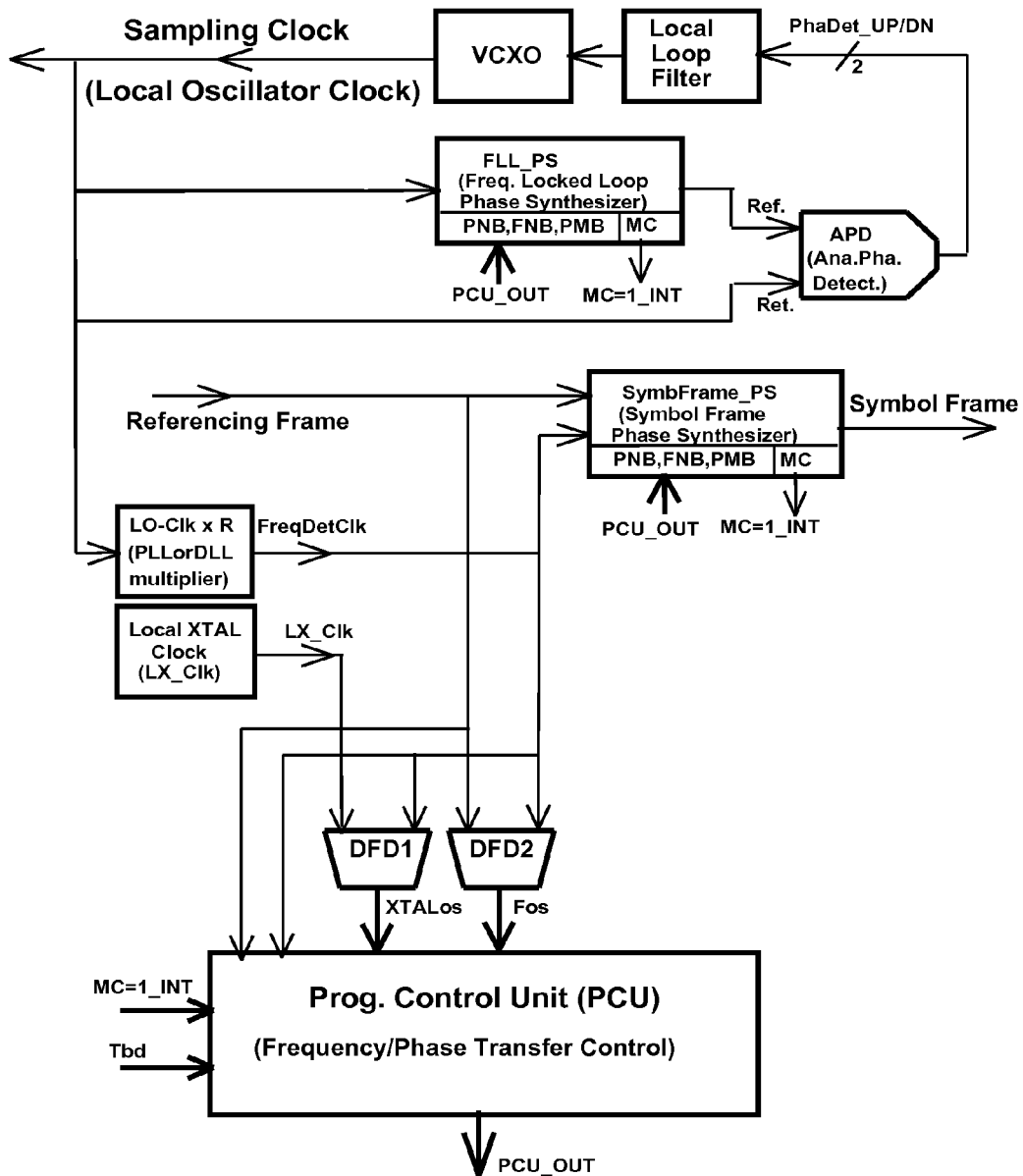
FIG.18 High Accuracy FLPS
