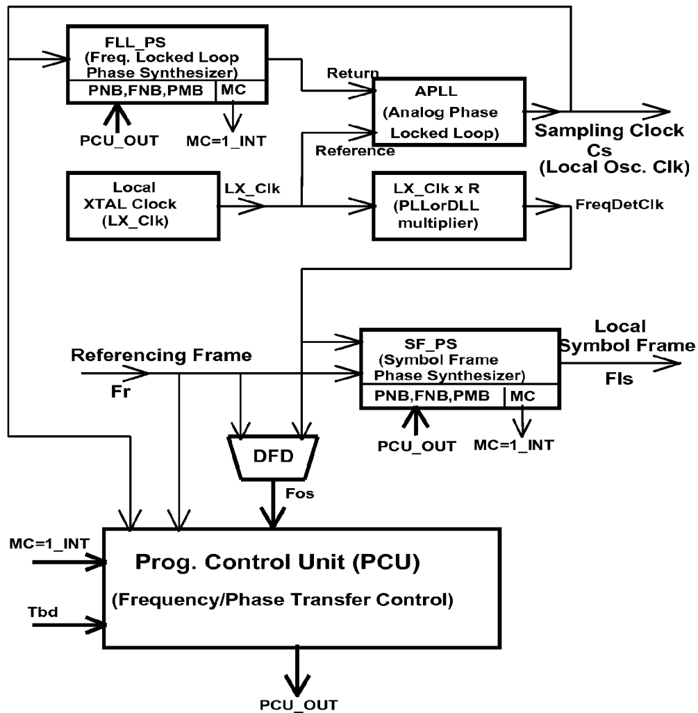
FIG.16 FLPS with Freq. Detector using XTAL clock
