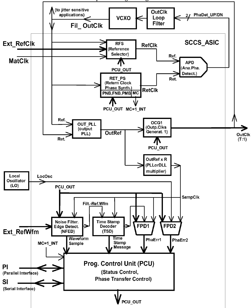
FIG.3 Heterodyne Timing Configuration of SCCS
