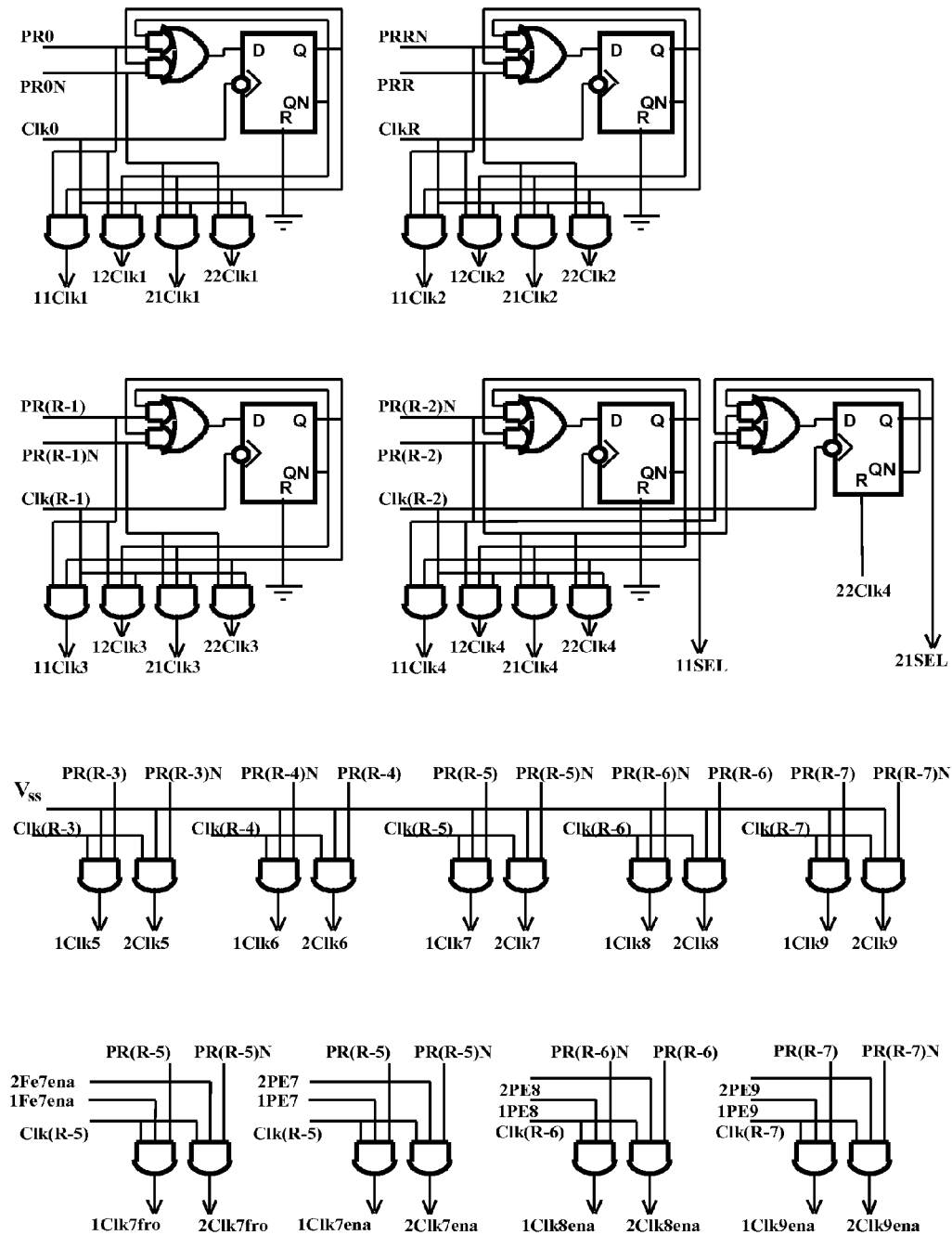
FIG.9 Sequential Clocks Generation for the NFED(SCG NFED)
