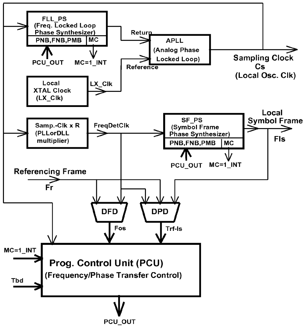
FIG.17 FLPS with Improved Stability
