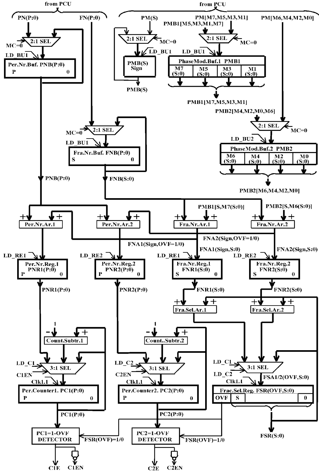
FIG.6 Synchronous Sequential Phase Processor (SSPP)
