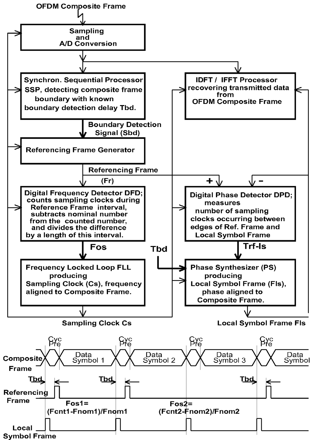
FIG.14 Synchronization System with Improved Stability
