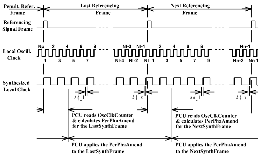
FIG.19B Timing of Direct FLPS
