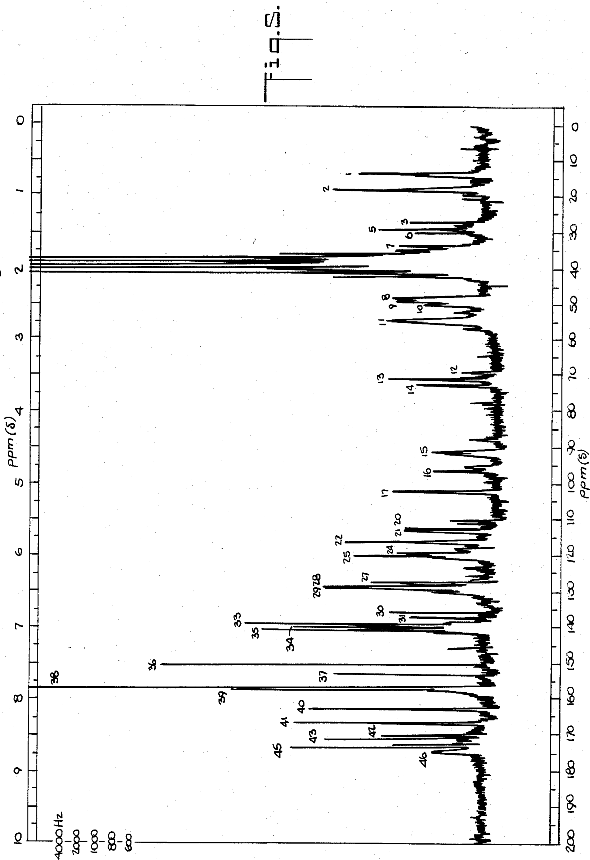
LL-802964X CARBON-13 NUCLEAR MAGNETIC RESONANCE SPECTRUM IN d_6 -DMF 2 O
