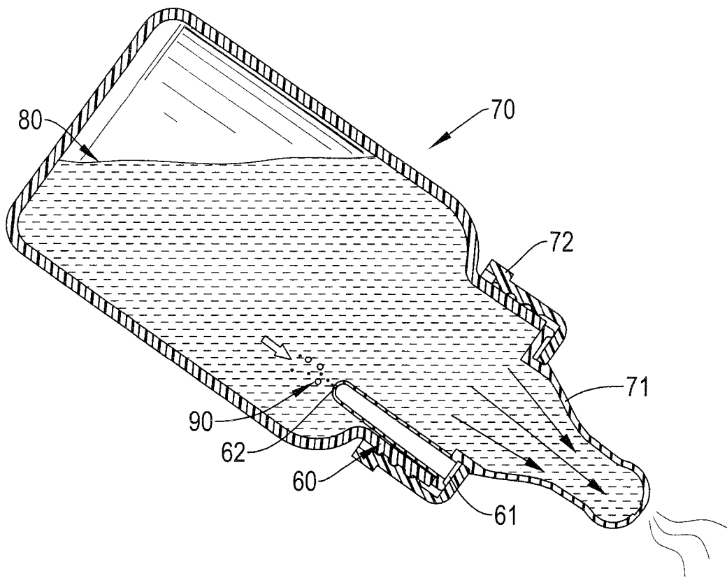
FIG. 11 PRIOR ART
