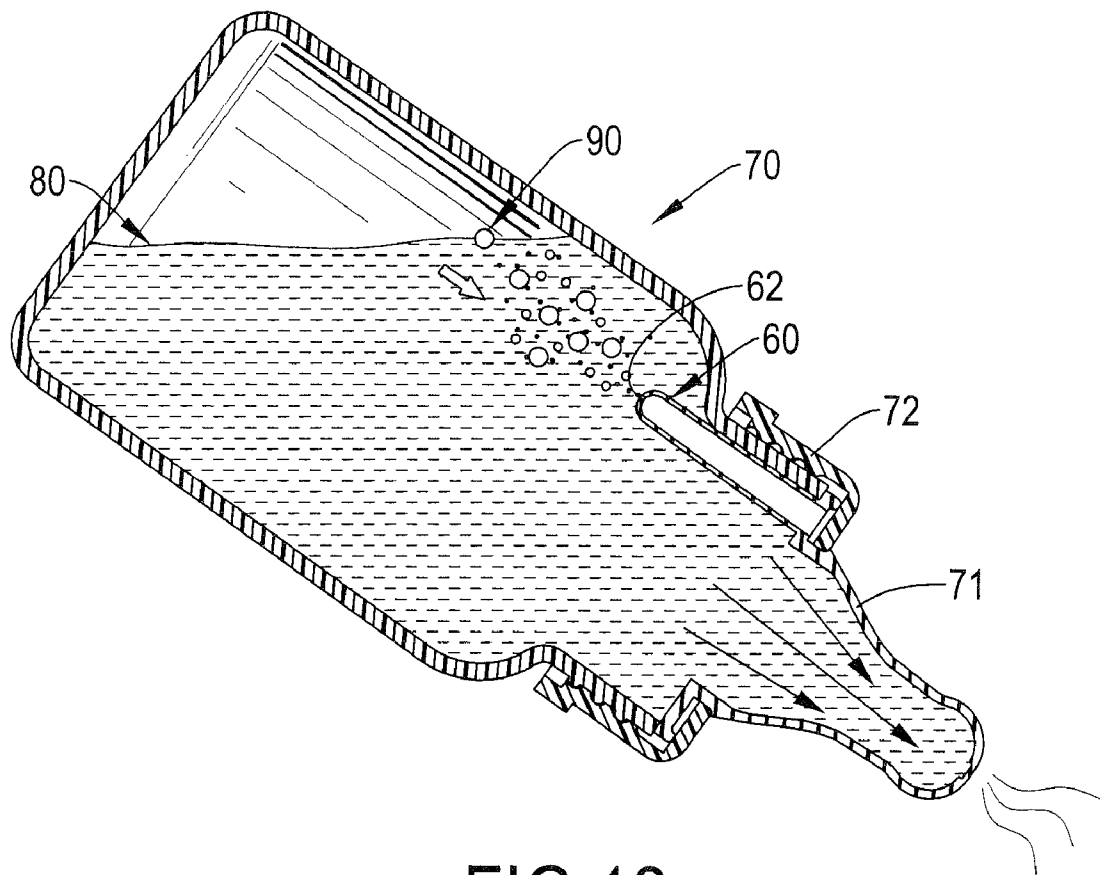
FIG. 12 PRIOR ART
