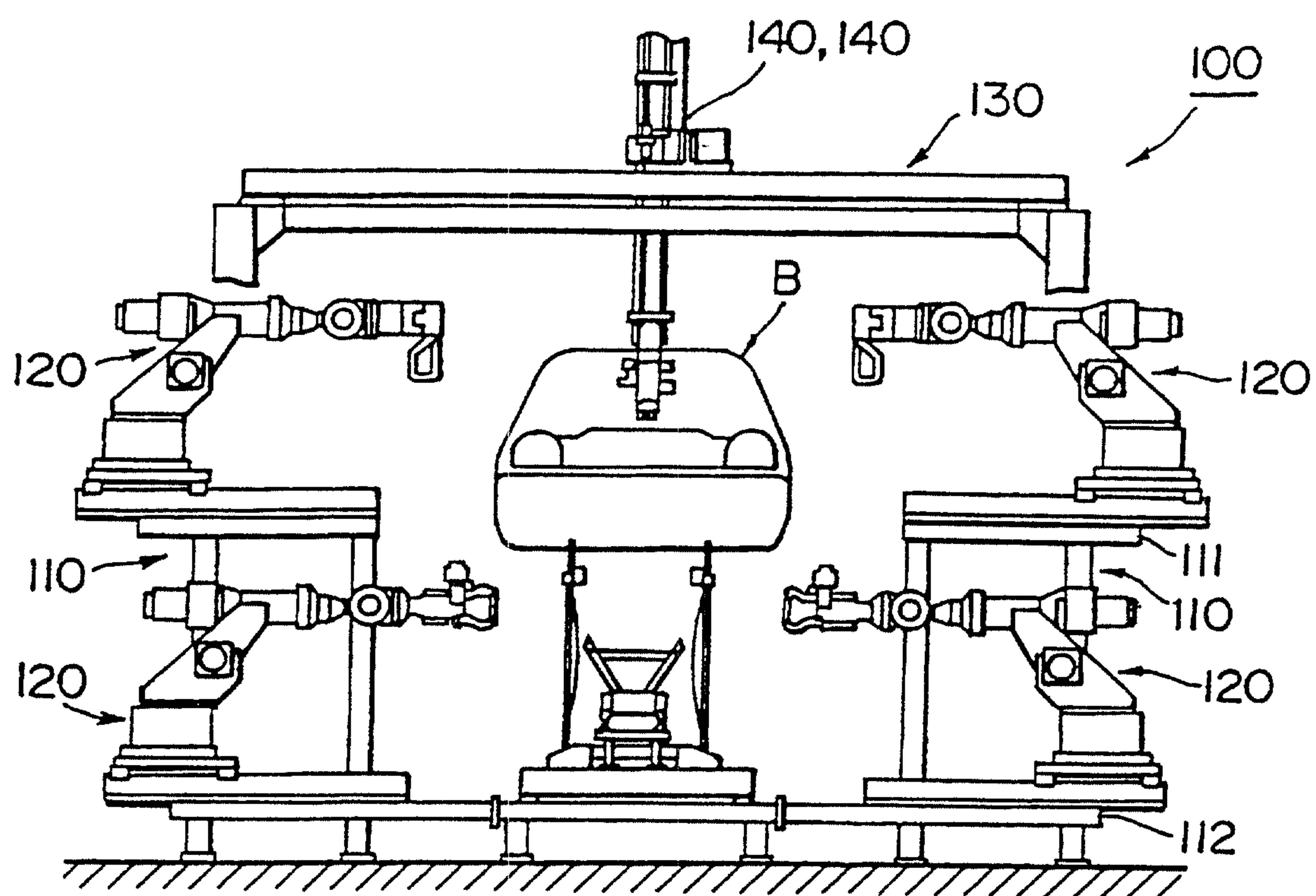
FIG. 16 PRIOR ART
