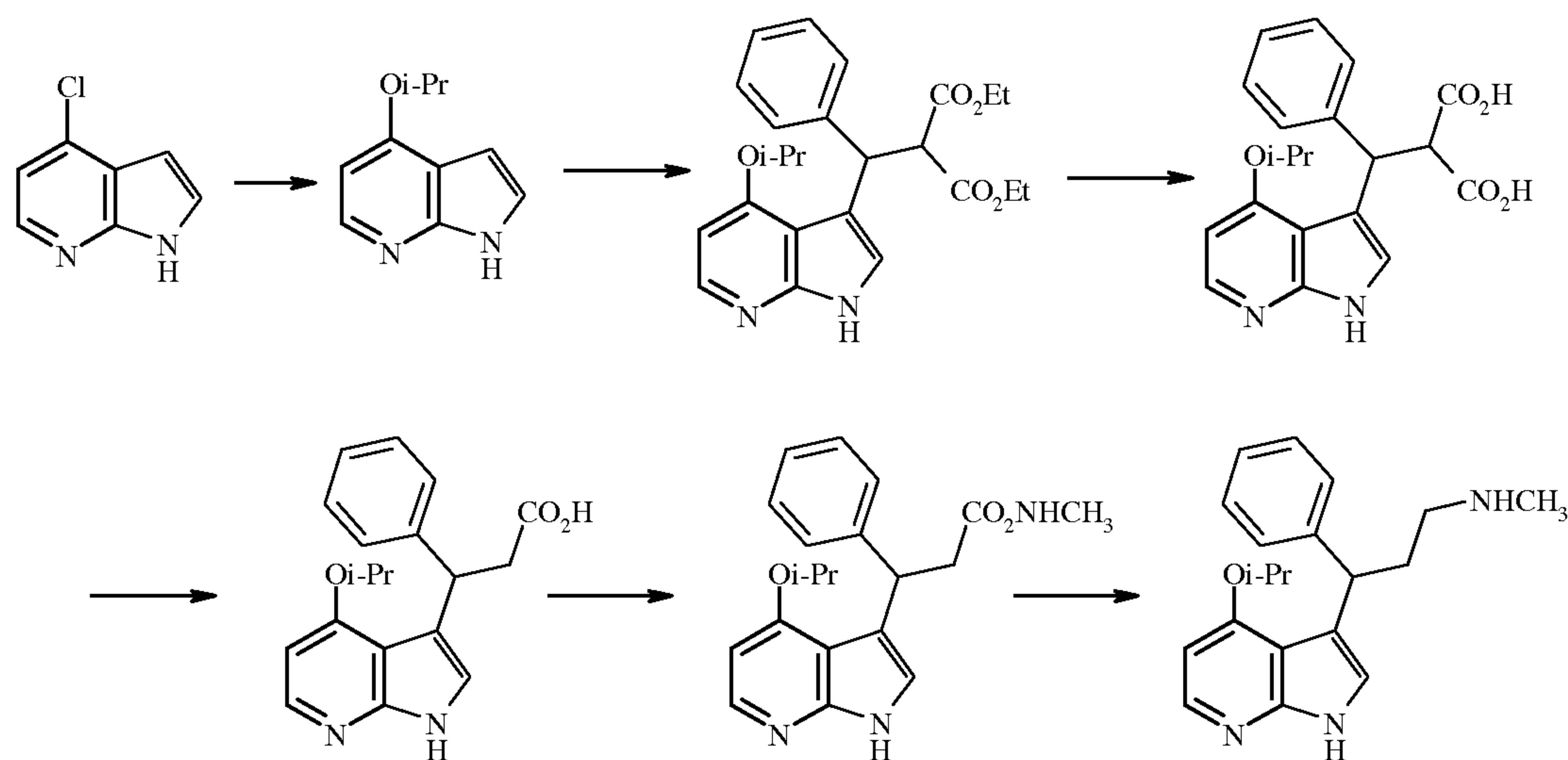
SCHEME CC
