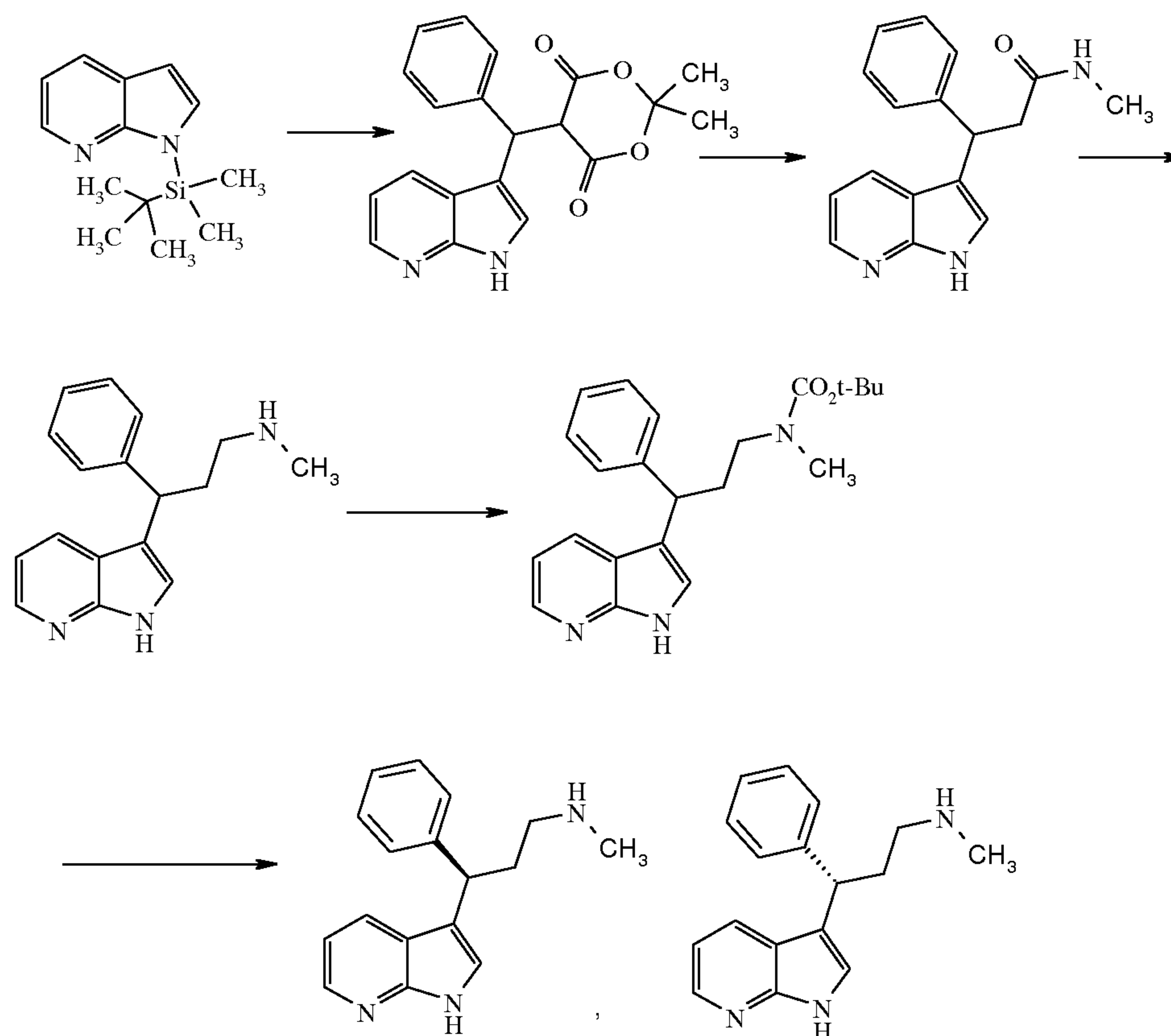
SCHEME G
