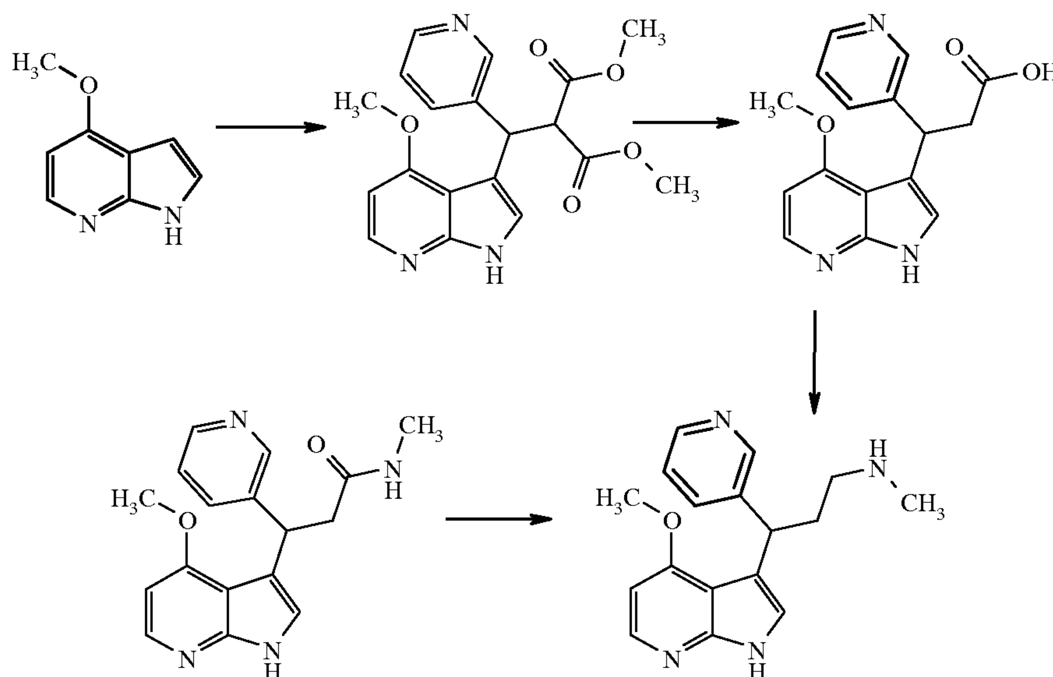
SCHEME J
