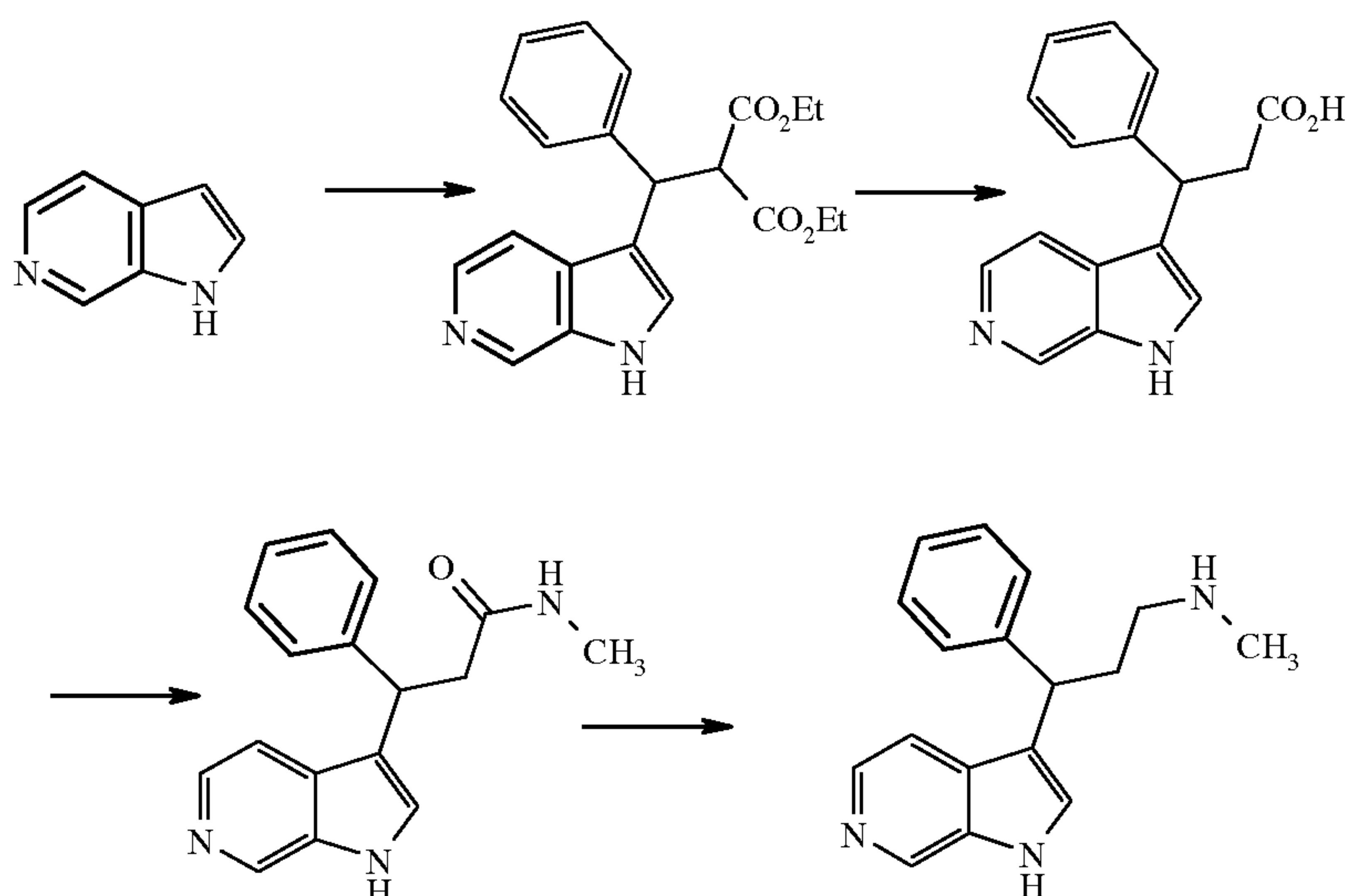
SCHEME L
