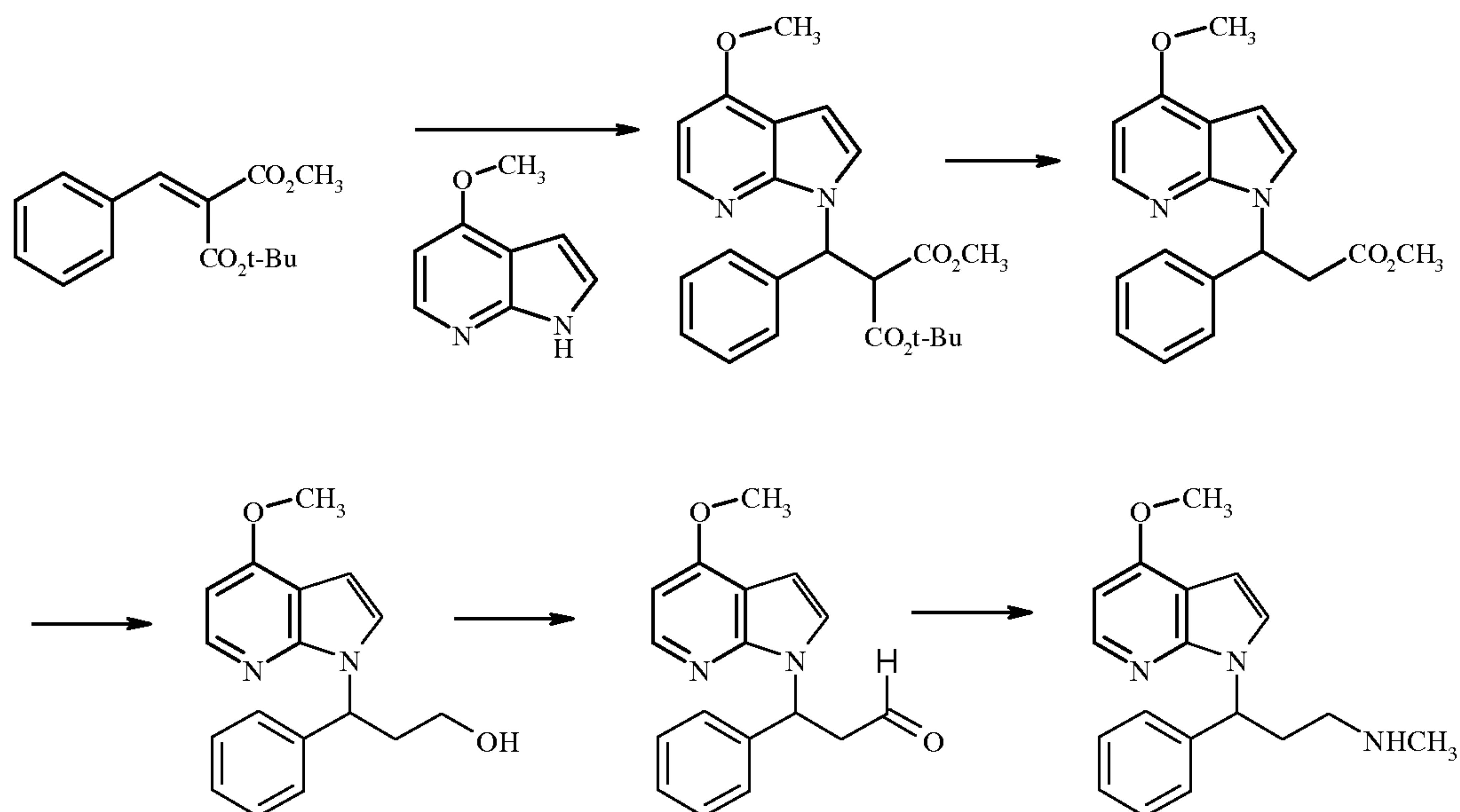
SCHEME AA
