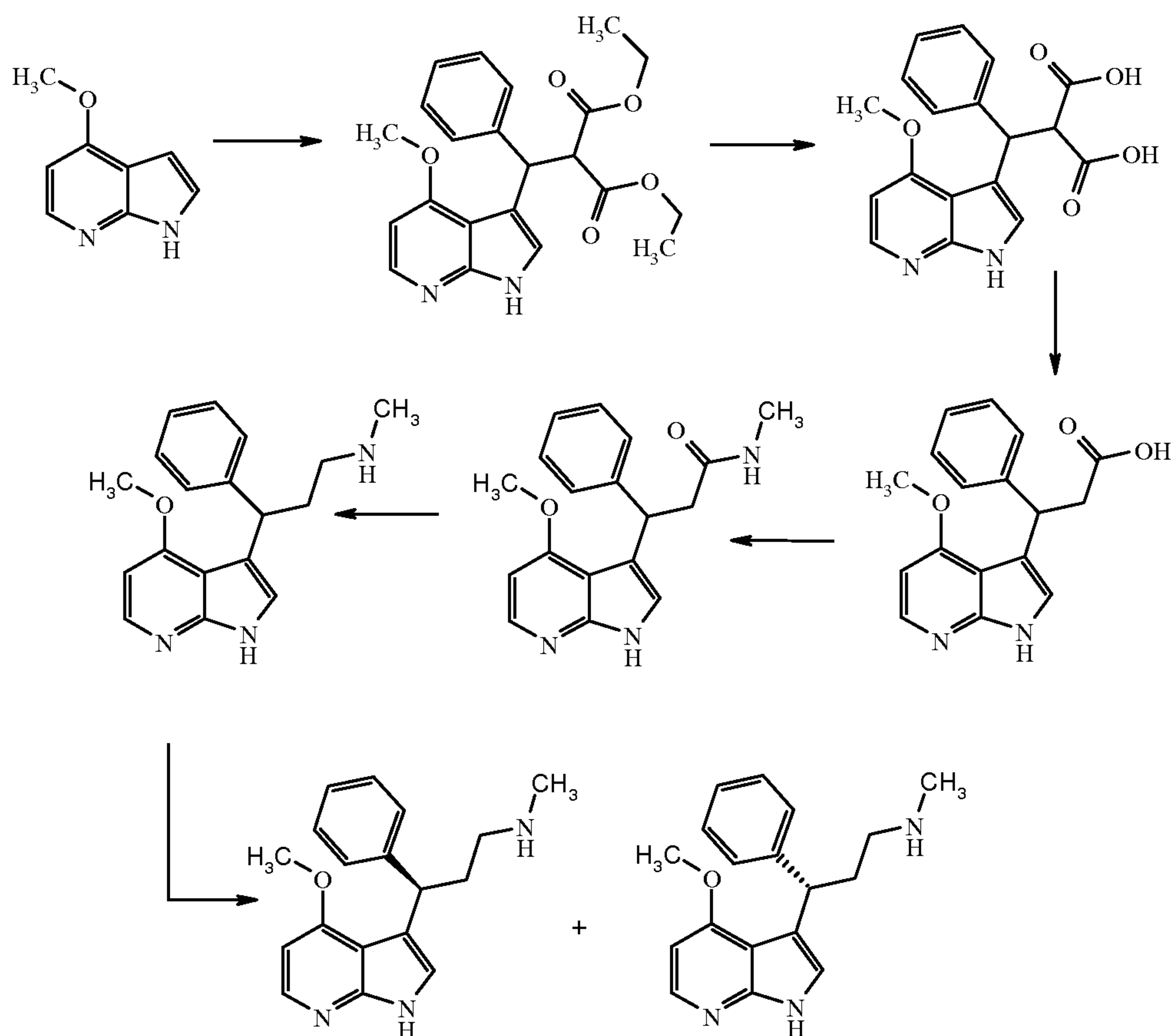
SCHEME I
