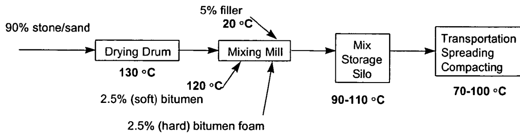
Figure 1: Schematic comparison of mix production routes. The percentage figures are given as percentage by mass
