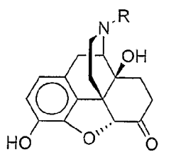
1a, R = CH 2 CH=CH 2 b, R = CH 2 C 3 H 5
