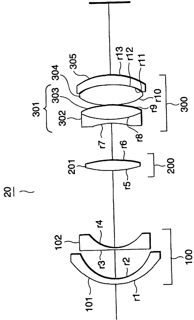
LENS CROSS-SECTIONAL VIEW (THIRD EMBODIMENT)
