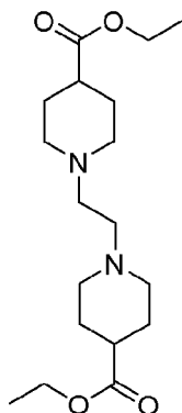
diethyl 1,1'-(ethane-1,2-diyl)bis(piperidine-4-carboxylate)
