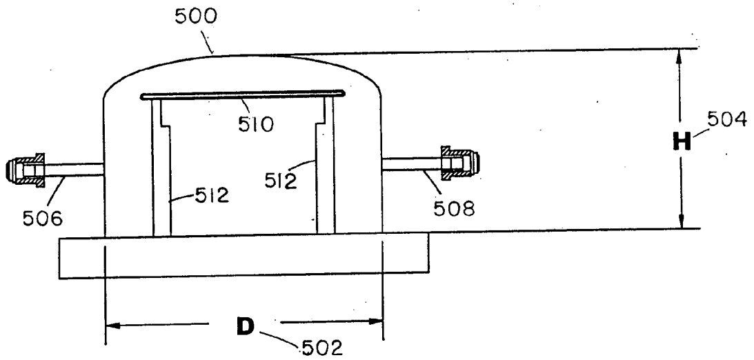
Wafer Chamber
