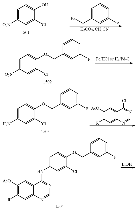
Scheme 15
