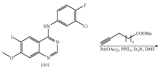
Scheme 11
