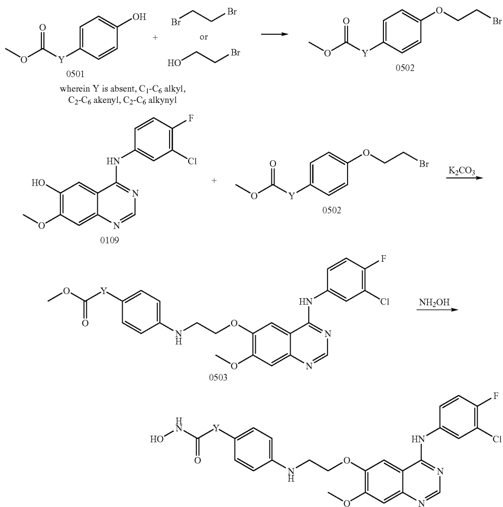
Scheme 5
