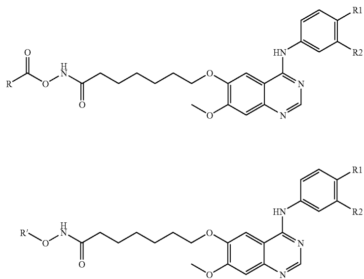
Scheme 9
