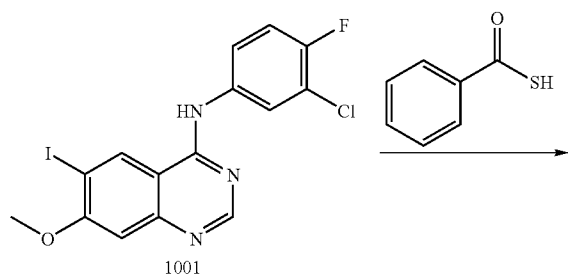
Scheme 12
