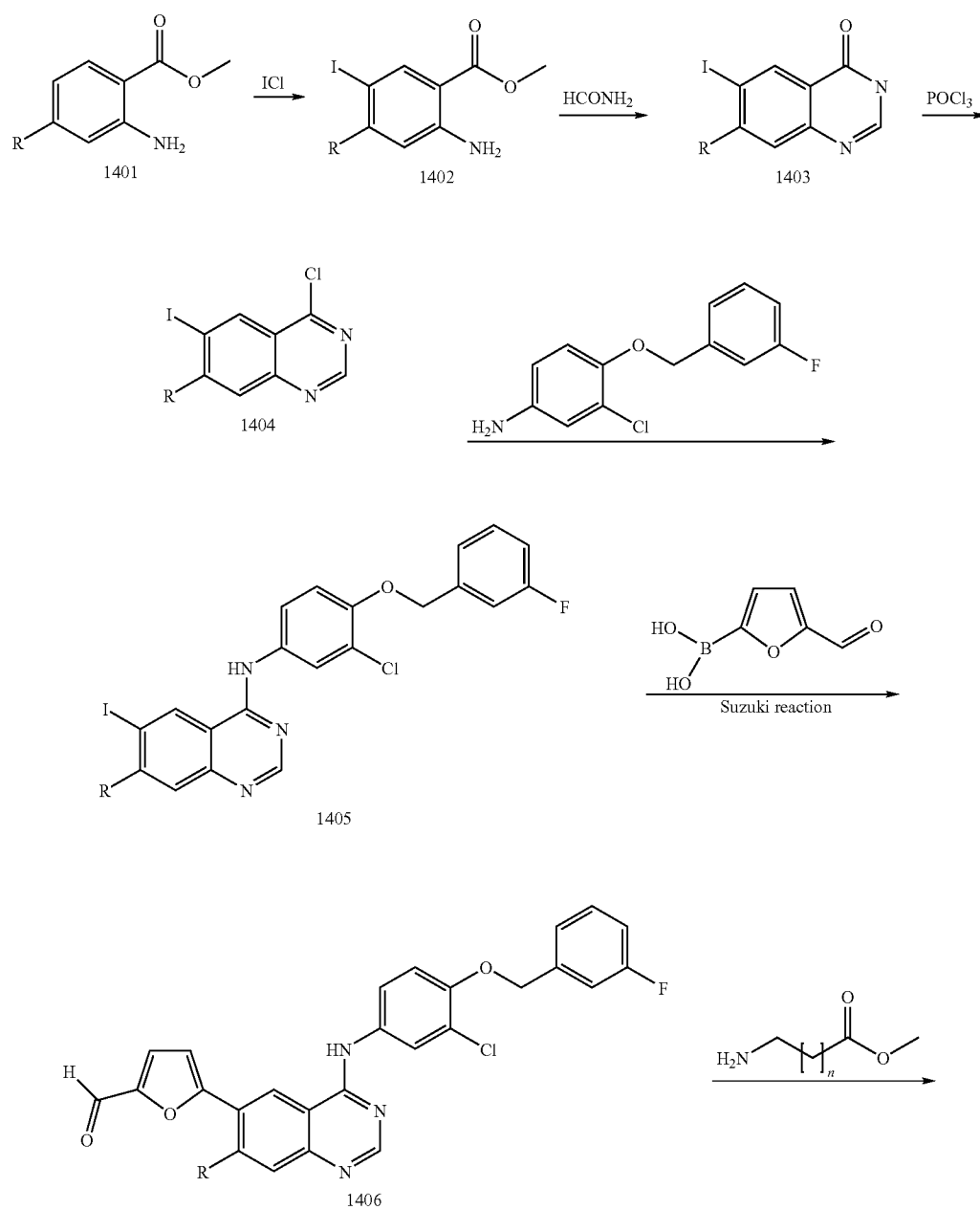
Scheme 14
