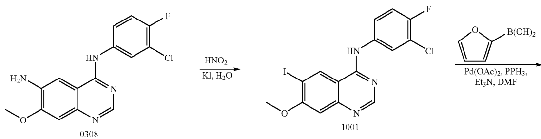
Scheme 10
