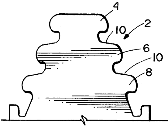
Fig. 1 (PRIOR ART)
