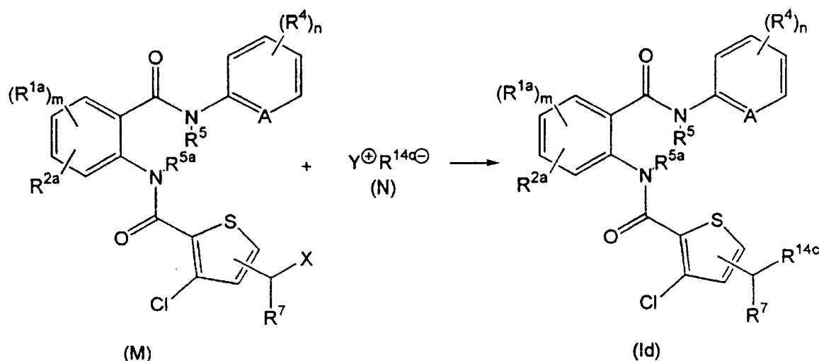
Reaction Scheme 4
