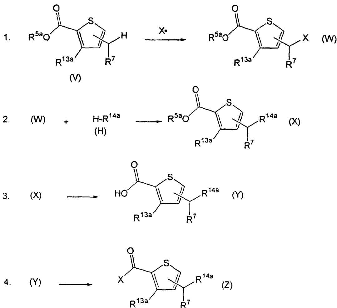
Reaction Scheme 11
