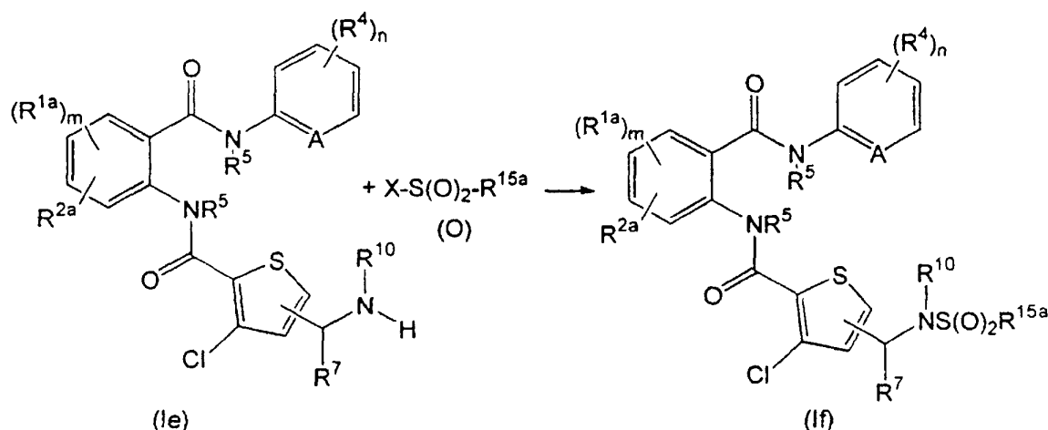
Reaction Scheme 5
