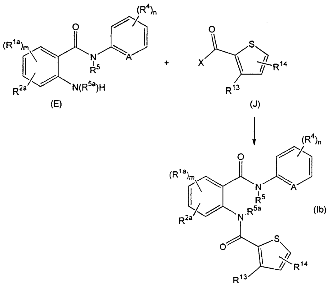
Reaction Scheme 2
