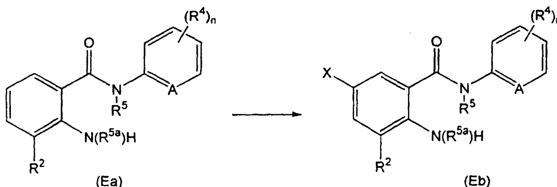
Reaction Scheme 18
