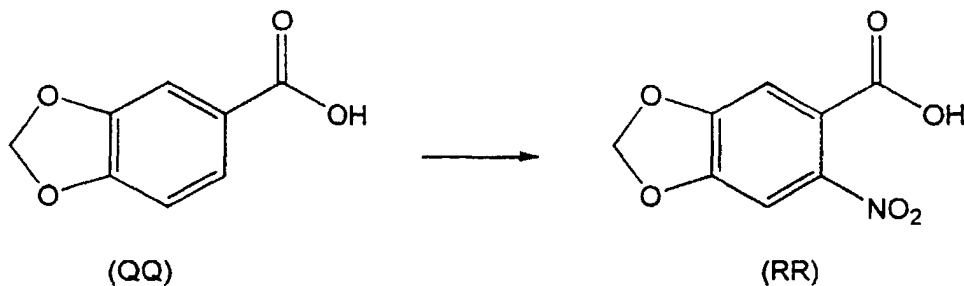
Reaction Scheme 22
