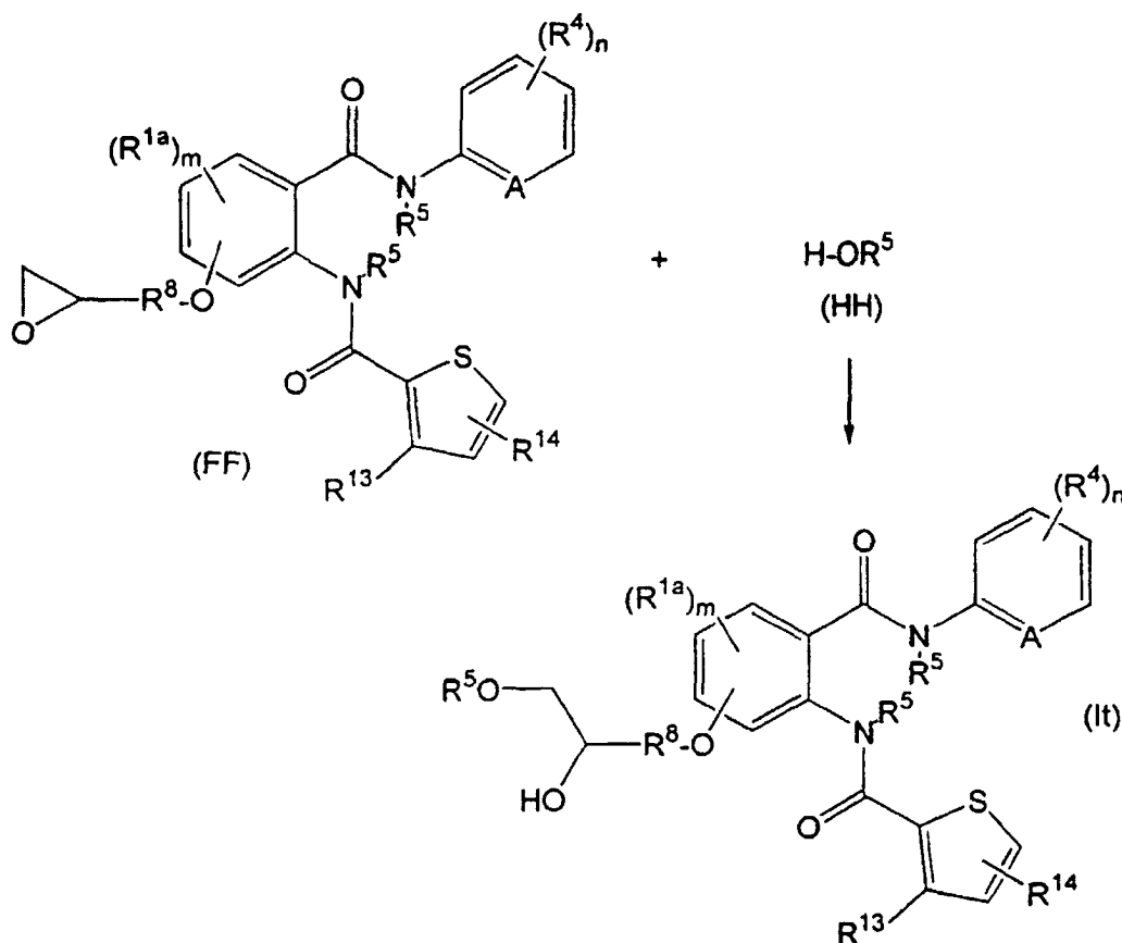
Reaction Scheme 15
