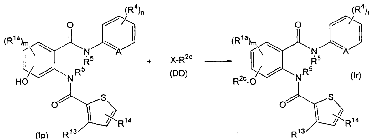
Reaction Scheme 13
