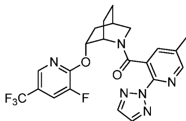
Example 437: ((1S,4R,6R)-6-((3-fluoro-5-(trifluoromethyl)pyridin-2-yl)oxy)-2-azabicyclo[2.2.2]octan-2-yl)(5-methyl-2-(2H-1,2,3-triazol-2-yl)pyridin-3-yl)methanone.
