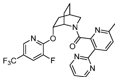
Example 435: ((1S,4R,6R)-6-((3-fluoro-5-(trifluoromethyl)pyridin-2-yl)oxy)-2-azabicyclo[2.2.2]octan-2-yl)(6-methyl-3-(pyrimidin-2-yl)pyridin-2-yl)methanone.
