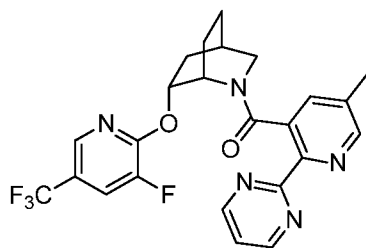
Example 436: ((1S,4R,6R)-6-((3-fluoro-5-(trifluoromethyl)pyridin-2-yl)oxy)-2-azabicyclo[2.2.2]octan-2-yl)(5-methyl-2-(pyrimidin-2-yl)pyridin-3-yl)methanone.
