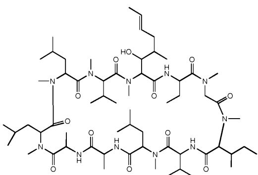
NIM-811, 3
