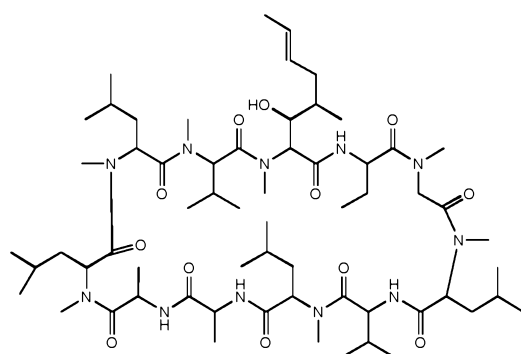
Cyclosporine A, 1
