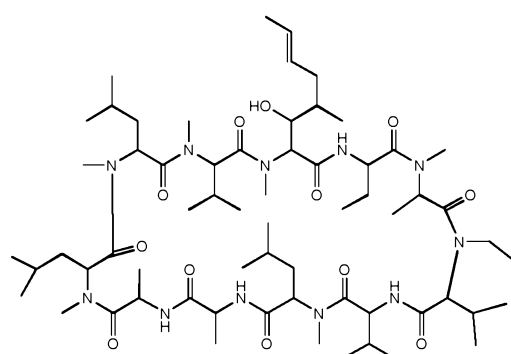
DEBIO-025, 2
