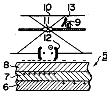
FIG. 4 (II) (PRIOR ART)
