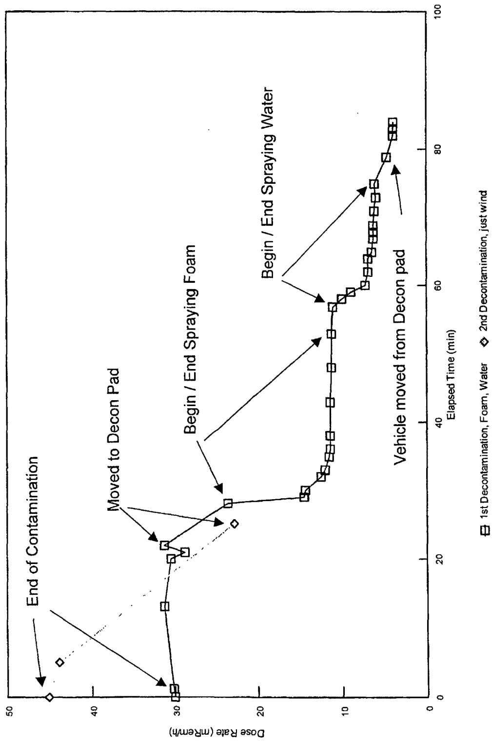
Fig. 15 Nuclear Particle Decontamination
