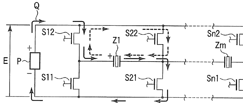
FIG. 1 (Related Art)
