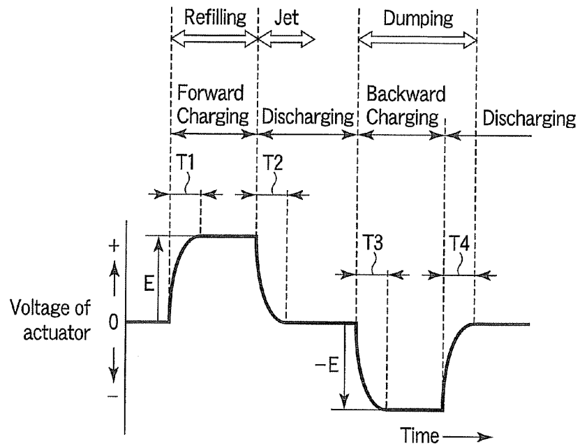
FIG. 2 (Related Art)
