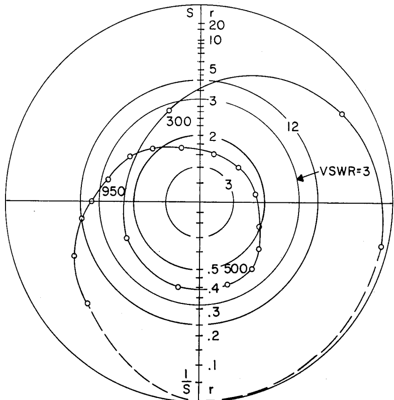
FIGURE 6 INPUT IMPEDANCE 3:1 FREQ BAND
