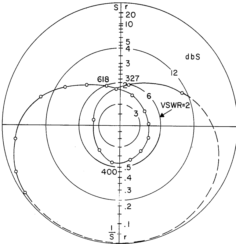
FIGURE 5 INPUT IMPEDANCE 2:1 FREQ BAND
