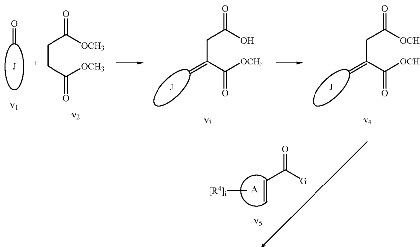
Reaction Sequence N
