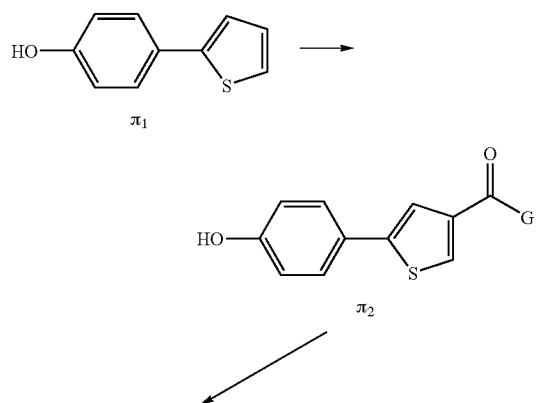
Reaction Sequence P
