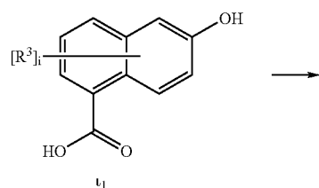
Reaction Sequence I
