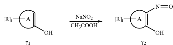
Reaction Sequence G
