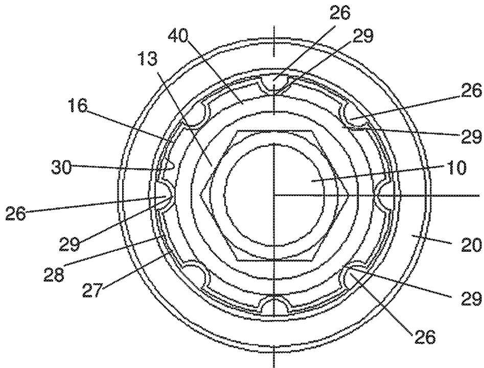
Figure 3 section A-A
