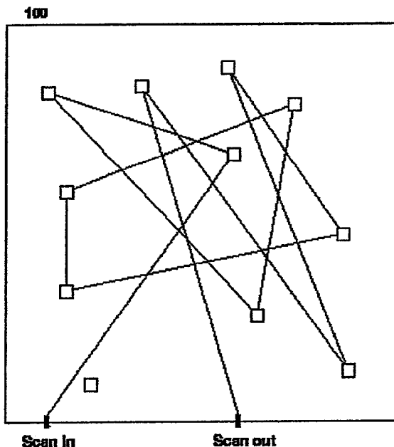
Initial (bad) scan chain order
