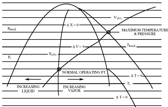
SIZING PROCESS ON PRESSURE ENTHALPY-DIAGRAM
