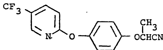
Compound 76 (oil)
