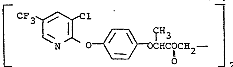
Compound 77 (oil)
