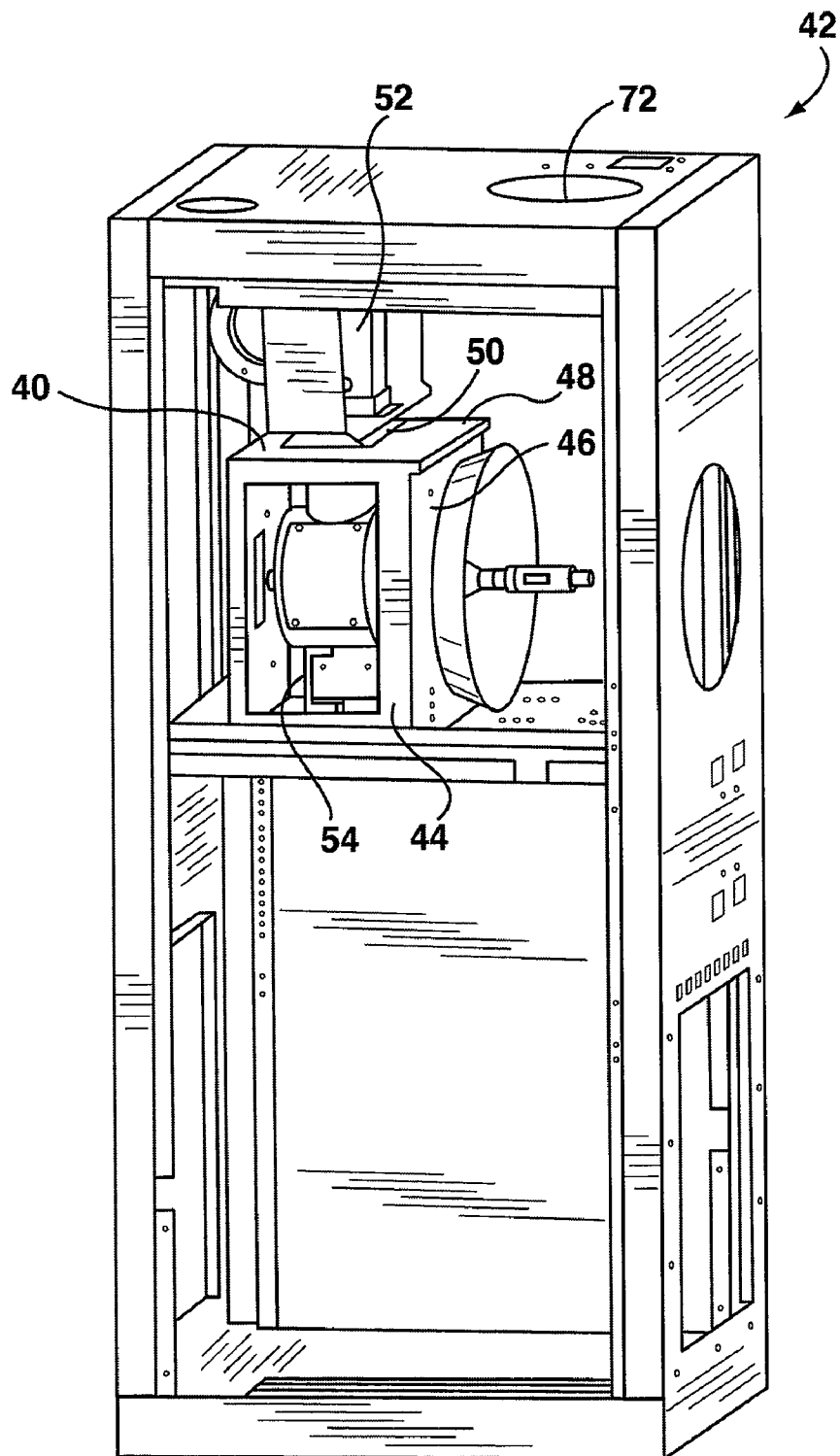
FIG. 3 (Prior Art)
