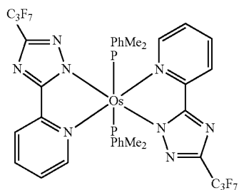
Os(hptz) 2 (PPhMe 2 ) 2
