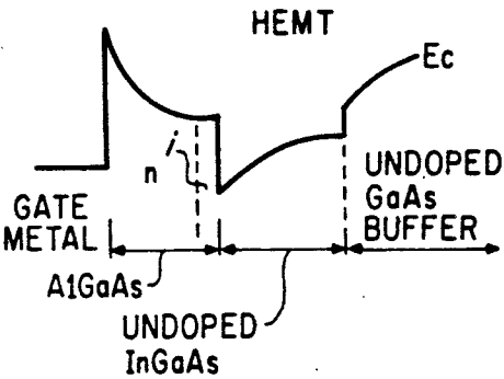
Fig. 2c PRIOR ART
