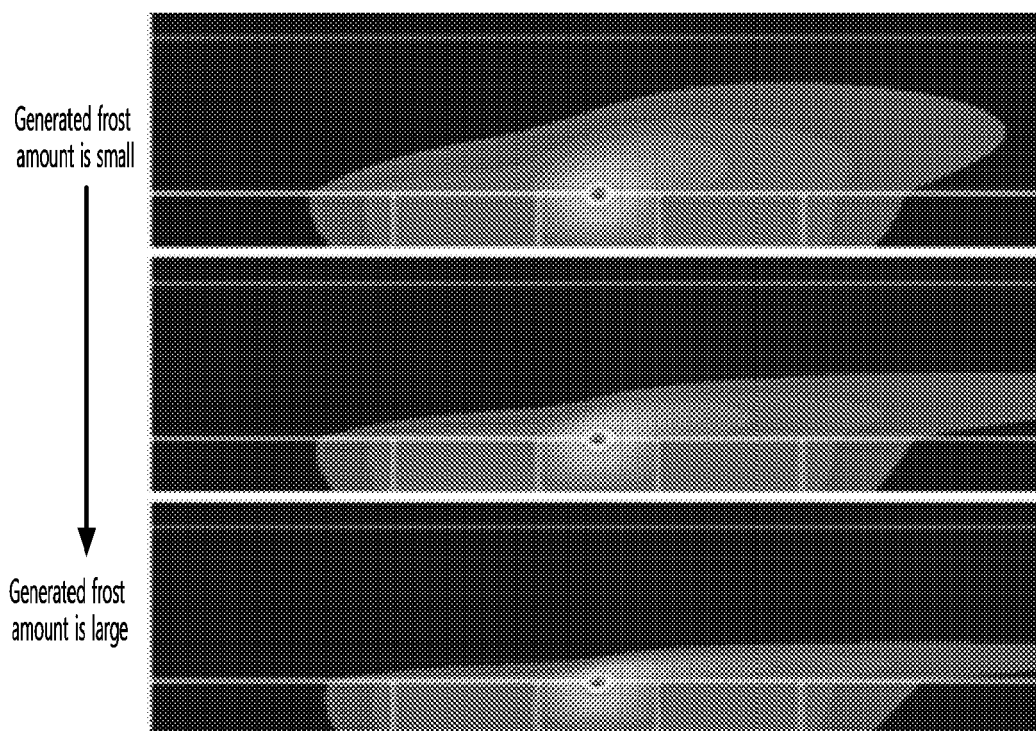
Thermal flow simulation depending on flow rate
