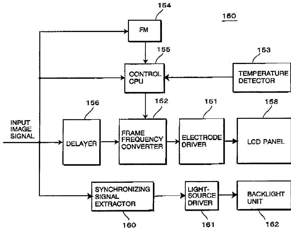
FIG. 2 PRIOR ART
