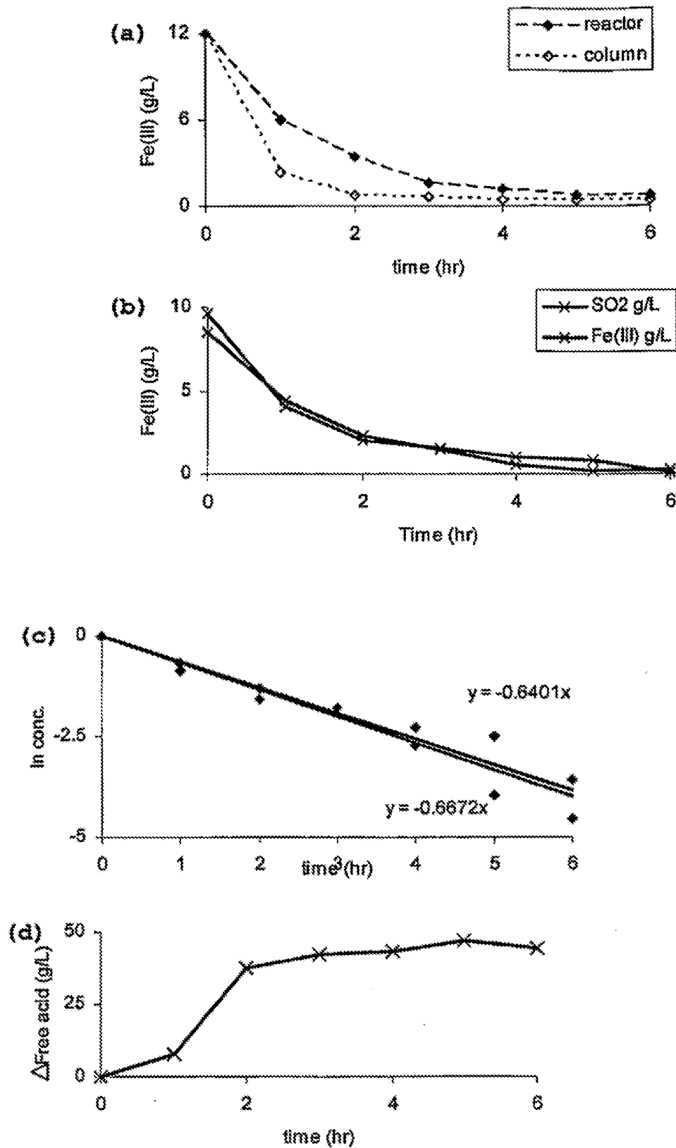
Figure 2: A series of graphs obtained from each \text{SO}_2 - Fe (III) reduction experimental run in Example 1.
