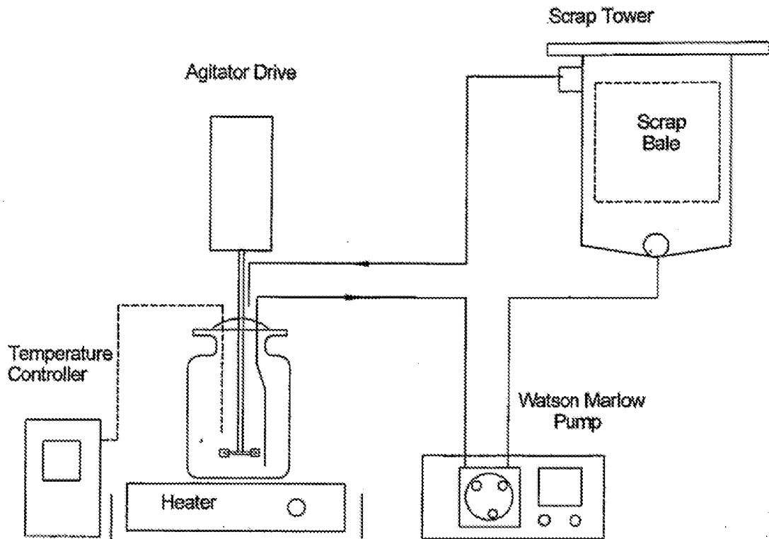
Figure 4 - Iron Reduction Experimental Set Up for Example
